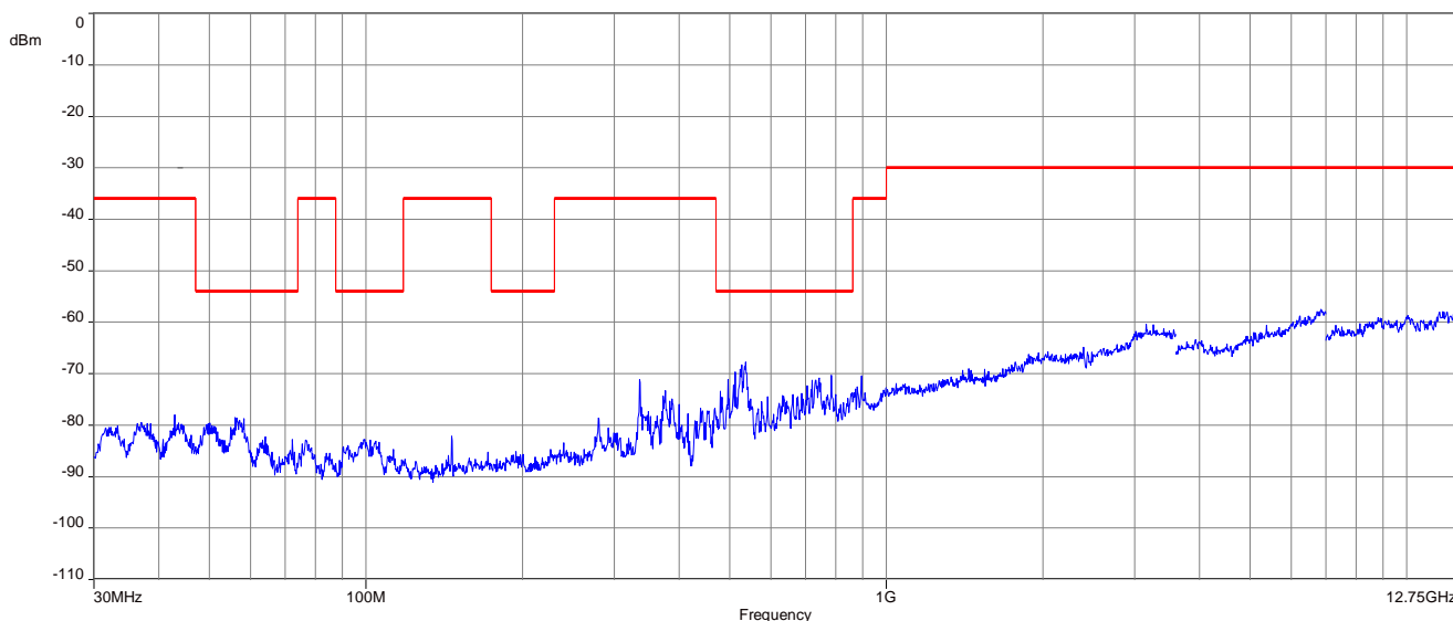
Plot 2: 30 MHz to 12.75 GHz, High channel, 1 Msps
