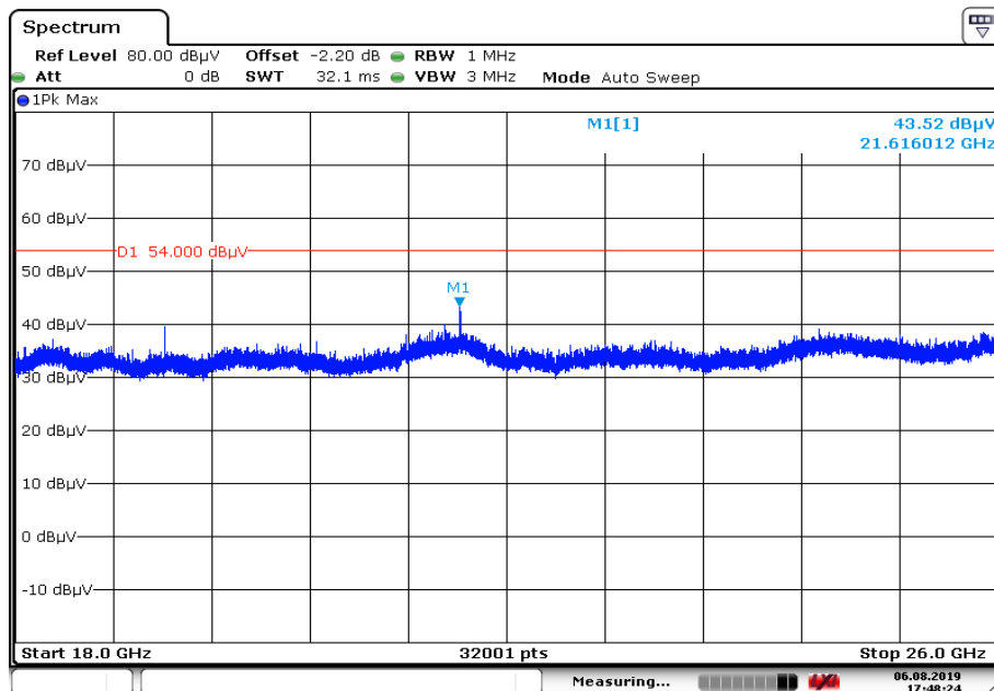
Plot 2: 18 GHz to 26 GHz, TX mode, 2402 MHz, vertical & horizontal polarization, 1 Msp
