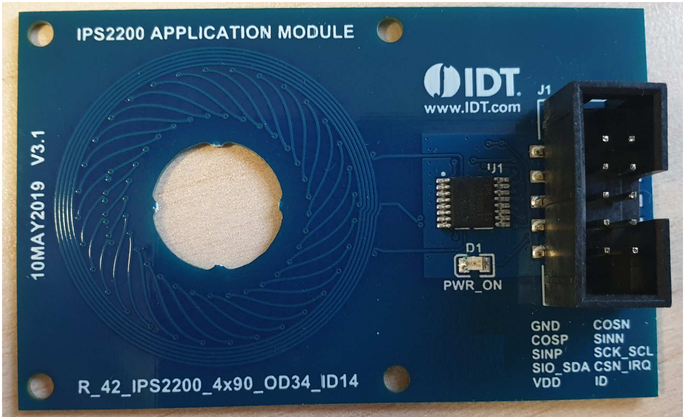
Figure 1. Sensor Board
