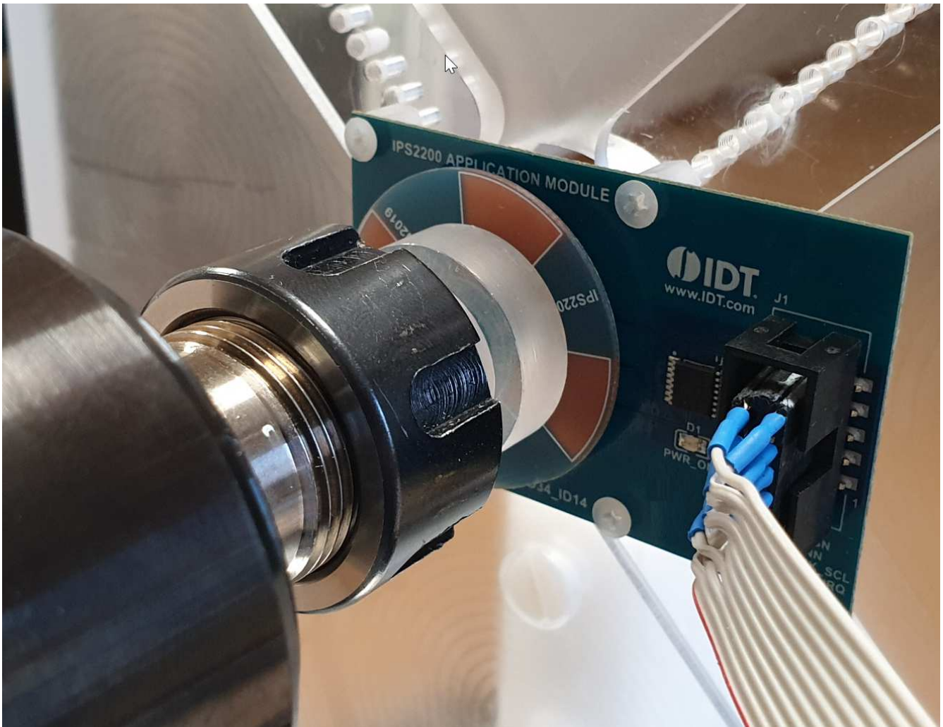
Figure 3. Setup
