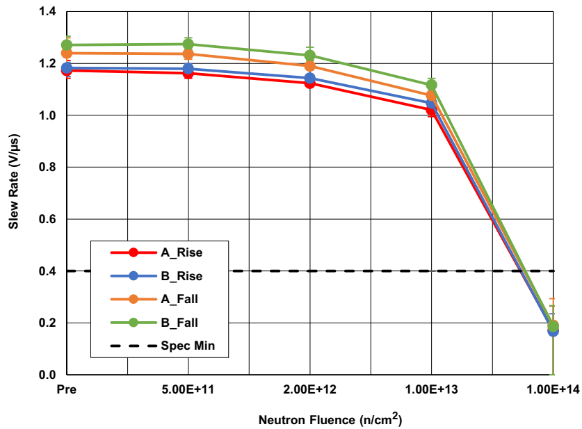
Figure 13. ISL70218SEH Slew Rate (SR), Channels A and B, with V_S = 15V , A_V = 1 , R_L = 2k\Omega , following irradiation to each level. The error bars (if visible) represent the minimum and maximum measured values. The SMD limit is 0.4V/µs.
