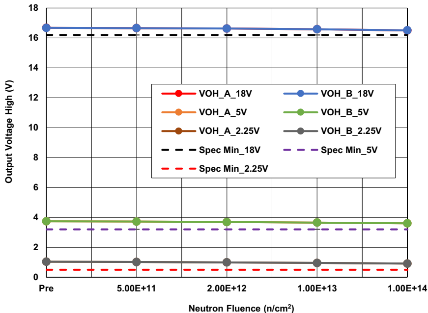
Figure 1. ISL70219ASEH Output Voltage High (V OH ), Channels A and B, with V S = ±18V, ±5V, and ±2.25V, R L = 10kΩ, following irradiation to each level. The error bars (if visible) represent the minimum and maximum measured values. The SMD limits are 16.2V minimum for V S = ±18V, 3.2V minimum for V S = ±5V, and 0.5V minimum for V S = ±2.25V.
