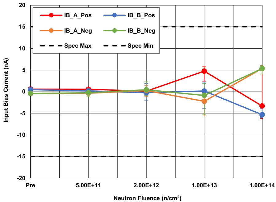
Figure 7. ISL70219ASEH Input Bias Current (I B ), Channels A and B, with V S = ±18V, following irradiation to each level. The error bars (if visible) represent the minimum and maximum measured values. The SMD limits are -15nA minimum and 15nA maximum.
