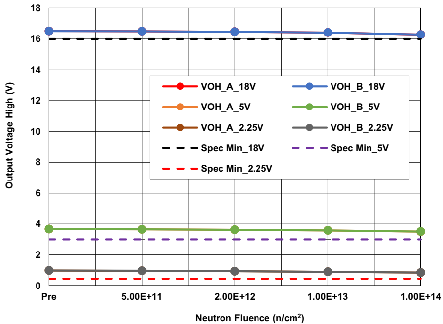
Figure 2. ISL70219ASEH Output Voltage High (V OH ), Channels A and B, with V S = ±18V, ±5V, and ±2.25V, R L = 2kΩ, following irradiation to each level. The error bars (if visible) represent the minimum and maximum measured values. The SMD limits are 16V minimum for V S = ±18V, 3V minimum for V S = ±5V, and 0.45V minimum for V S = ±2.25V.
