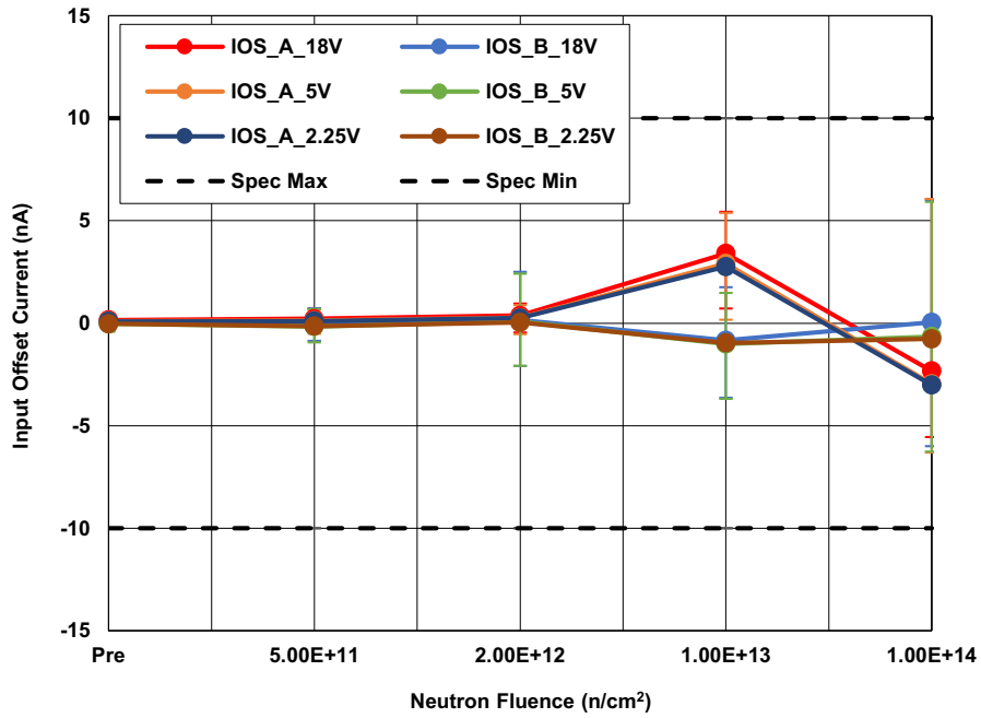
Figure 10. ISL70219ASEH Input Offset Current ( I_{OS} ), Channels A and B, with V_S = \pm 18V, \pm 5V, and \pm 2.25V , following irradiation to each level. The error bars (if visible) represent the minimum and maximum measured values. The SMD limits are -10nA minimum and 10nA maximum.
