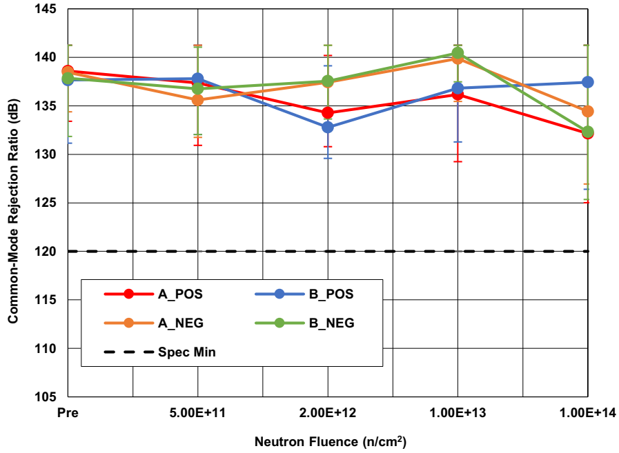
Figure 16. ISL70219ASEH Common-Mode Rejection Ratio (CMRR), Channels A and B, with V_S = \pm 5V , following irradiation to each level. The error bars (if visible) represent the minimum and maximum measured values. The SMD limit is 120dB minimum.
