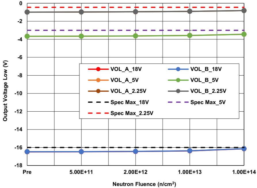
Figure 4. ISL70219ASEH Output Voltage Low ( V_{OL} ), Channels A and B, with V_S = \pm 18V, \pm 5V, and \pm 2.25V, R_L = 2k\Omega, following irradiation to each level. The error bars (if visible) represent the minimum and maximum measured values. The SMD limits are -16V maximum for V_S = \pm 18V, -3V maximum for V_S = \pm 5V, and -0.45V maximum for V_S = \pm 2.25V.
