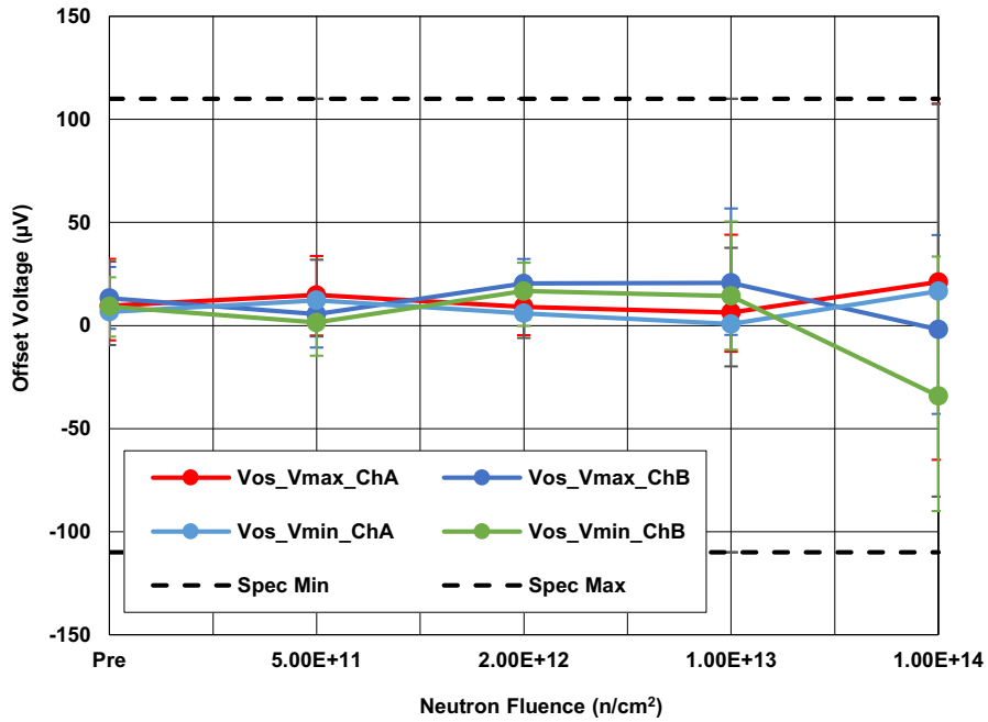
Figure 6. ISL70219ASEH Input Offset Voltage (V OS ), Channels A and B, with V S = ±18V and ±2.25V, following irradiation to each level. The error bars (if visible) represent the minimum and maximum measured values. The SMD limits -110µV minimum and 110µV maximum.
