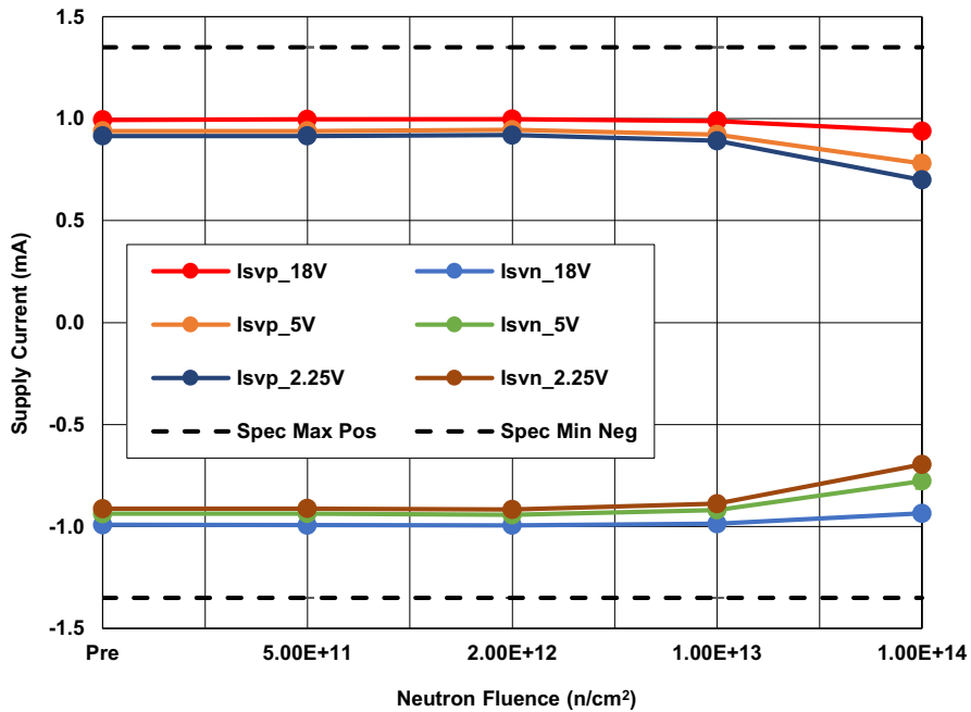
Figure 5. ISL70219ASEH Positive and Negative Supply Current ( I_{SVP} and I_{SVN} ), for Channels A + B, with V_S = \pm 18V, \pm 5V, and \pm 2.25V, following irradiation to each level. The error bars (if visible) represent the minimum and maximum measured values. The SMD limits are -1.35mA minimum and 1.35mA maximum.
