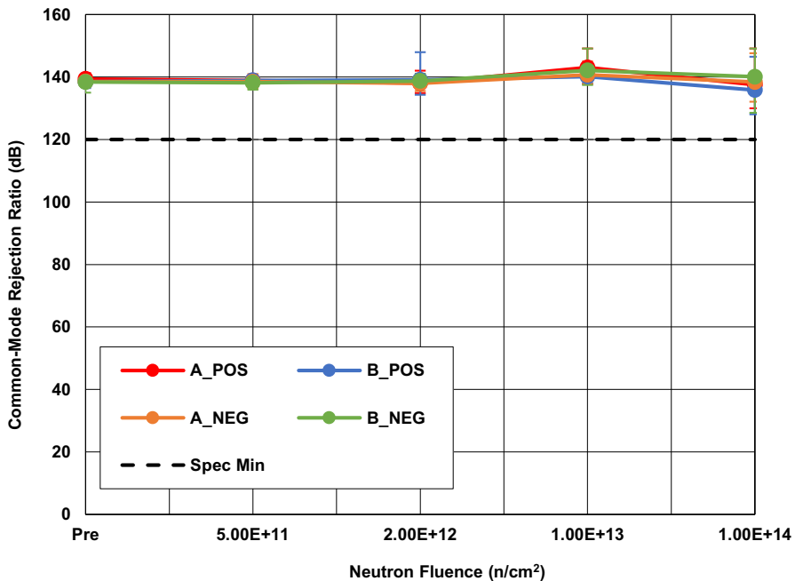
Figure 15. ISL70219ASEH Common-Mode Rejection Ratio (CMRR), Channels A and B, with V_S = \pm 18V , following irradiation to each level. The error bars (if visible) represent the minimum and maximum measured values. The SMD limit is 120dB minimum.
