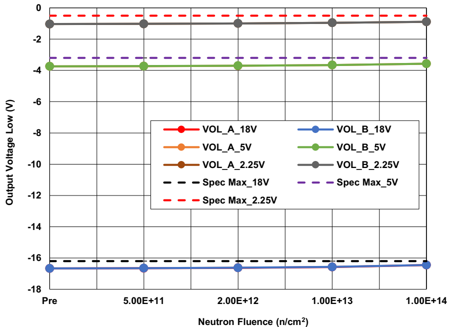
Figure 3. ISL70219ASEH Output Voltage Low (V OL ), Channels A and B, with V S = ±18V, ±5V, and ±2.25V, R L = 10kΩ, following irradiation to each level. The error bars (if visible) represent the minimum and maximum measured values. The SMD limits are -16.2V maximum for V S = ±18V, -3.2V maximum for V S = ±5V, and -0.5V maximum for V S = ±2.25V.
