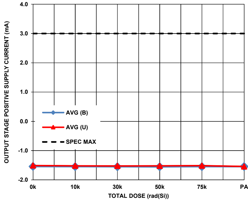
FIGURE 44. ISL70517SEH output stage positive supply current ( I_{C0} ) at \pm 18V , as a function of low dose rate irradiation for the Biased (B) (per Figure 1) and Unbiased (U) (all pins grounded) cases. The error bars represent the minimum and maximum measured values. The post-irradiation SMD limit is 3.0mA maximum.
