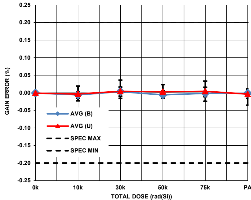
FIGURE 31. ISL70517SEH gain error with the input amplifier at \pm 4V and the output amplifier at \pm 1.5V , V_{OUT} = \pm 0.1V , R_{FB} = 121k , Gain = 1, as a function of low dose rate irradiation for the Biased (B) (per Figure 1) and Unbiased (U) (all pins grounded) cases. The error bars represent the minimum and maximum measured values. The post-irradiation SMD limits are -0.2% to 0.2%.
