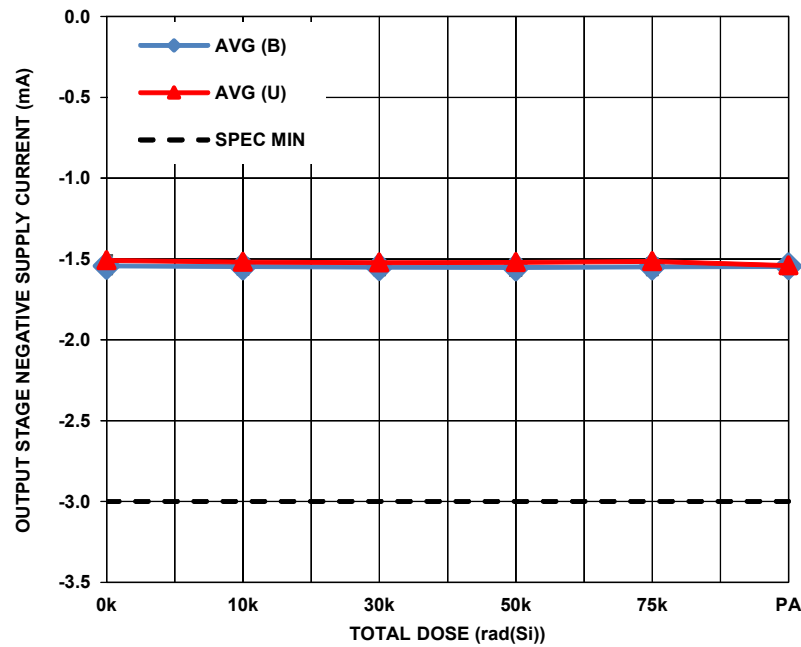
FIGURE 45. ISL70517SEH output stage negative supply current ( I_{E0} ) at \pm 18V , as a function of low dose rate irradiation for the Biased (B) (per Figure 1) and Unbiased (U) (all pins grounded) cases. The error bars represent the minimum and maximum measured values. The post-irradiation SMD limit is -3.0mA minimum.
