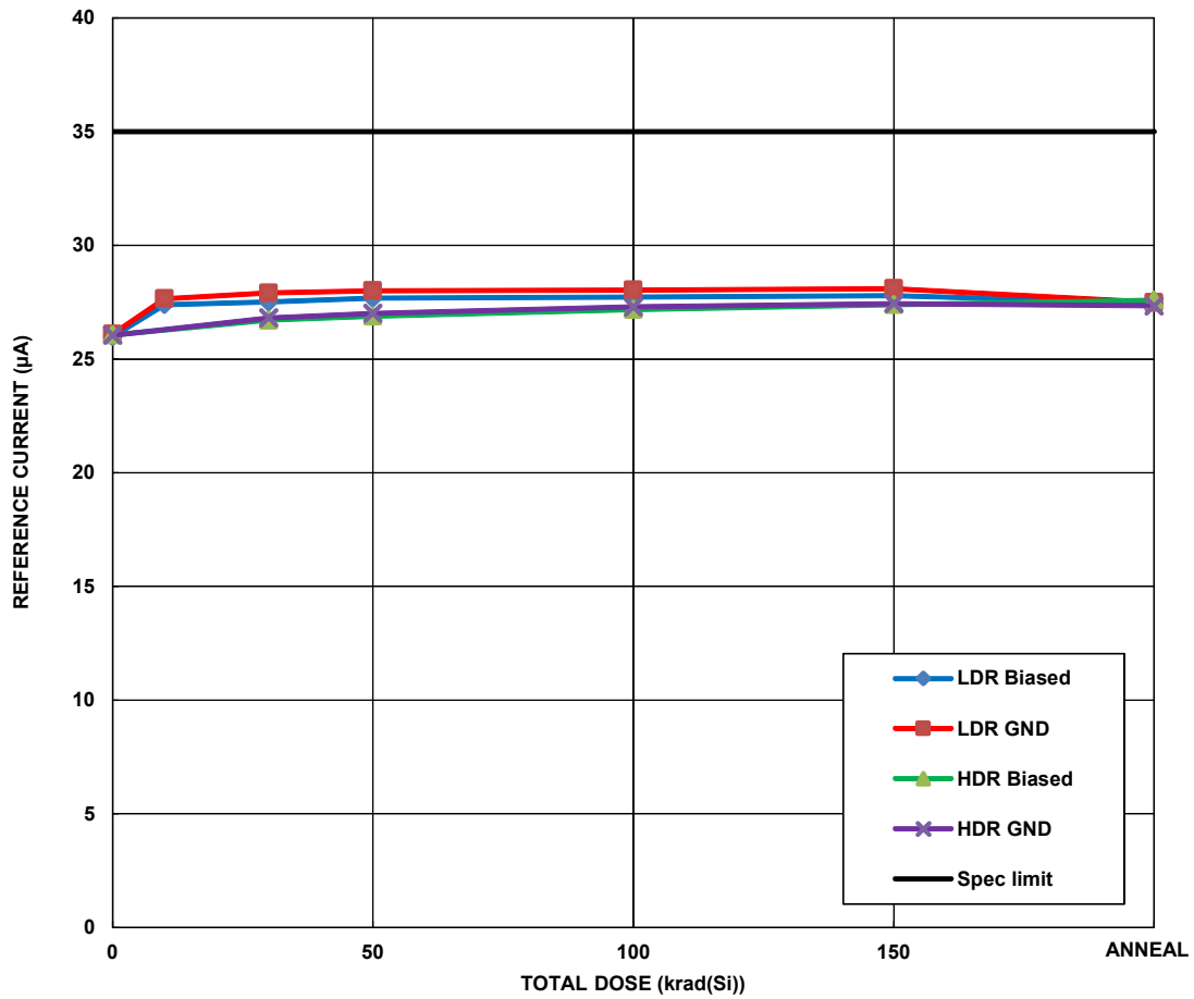
FIGURE 7. Median ISL71841SEH reference current as a function of total dose irradiation at high and low dose rate for the biased (per Figure 2) and unbiased (all pins grounded) cases. The low dose rate was 0.0085rad(Si)/s and the high dose rate was 69.7rad(Si)/s. Irradiations were followed by a 168-hour biased anneal at +100°C. Sample size for the low dose rate cells was 13 and sample size for the high dose rate cells was 4. The post-irradiation SMD limit is 35µA maximum.
