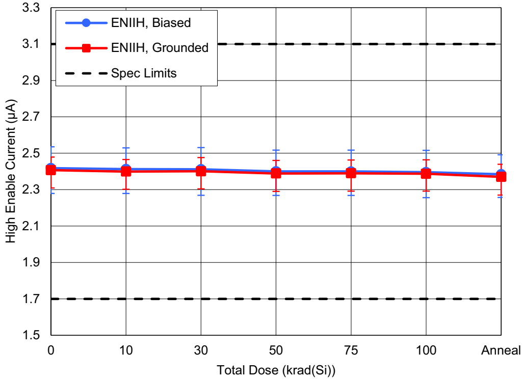
Figure 27. ISL73006SLH High Enable Current (EN IH ) as a function of LDR irradiation and anneal for biased and grounded configurations. The error bars (if visible) represent the minimum and maximum measured values. The datasheet limits are a minimum of 1.7μA and a maximum of 3.1μA.
