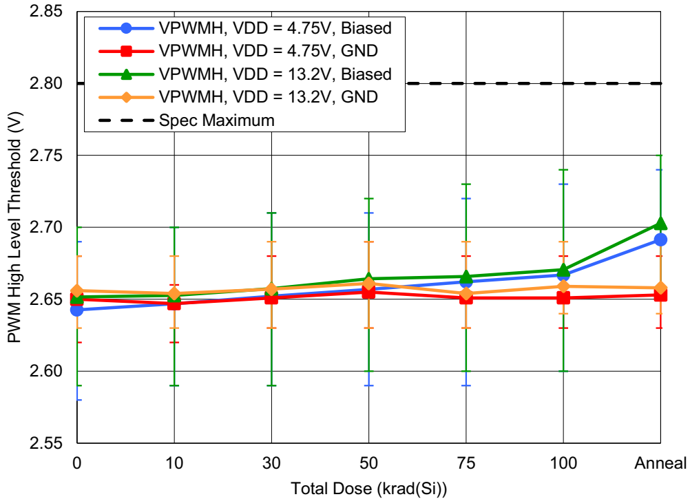
Figure 14. ISL73041SEH PWM high level threshold ( V_{PWMH} ) with V_{DD} = 4.75V or 13.2V as a function of LDR irradiation and anneal for biased and grounded configurations. The error bars (if visible) represent the minimum and maximum measured values. The datasheet limit is a maximum of 2.8V.
