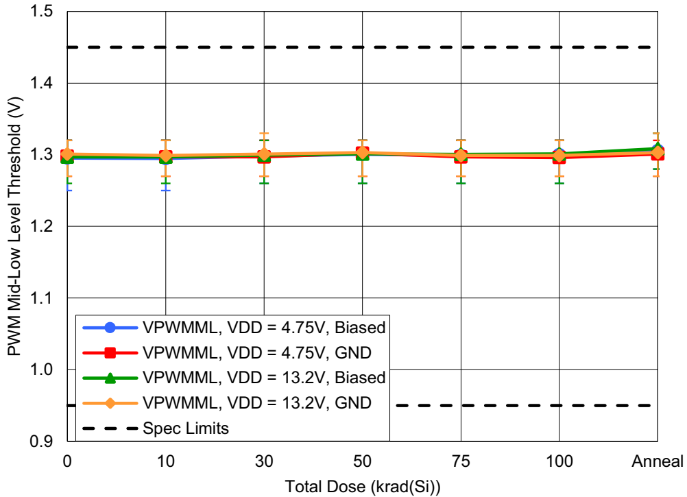
Figure 16. ISL73041SEH low mid-level threshold ( V_{PWML} ) with V_{DD} = 4.75V or 13.2V as a function of LDR irradiation and anneal for biased and grounded configurations. The error bars (if visible) represent the minimum and maximum measured values. The datasheet limits are a minimum of 0.95V and a maximum of 1.45V .
