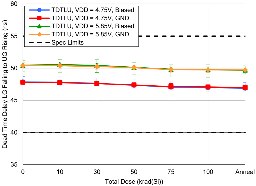
Figure 19. ISL73041SEH dead time delay, LG falling to UG rising ( t_{D\text{TDLU}} ) with V_{DD} = 4.75\text{V} or 5.85\text{V} , and with R_{DU} = R_{DL} = 10\text{k}\Omega to GND as a function of LDR irradiation and anneal for biased and grounded configurations. The error bars (if visible) represent the minimum and maximum measured values. The datasheet limits are a minimum of 40ns and a maximum of 55ns.
