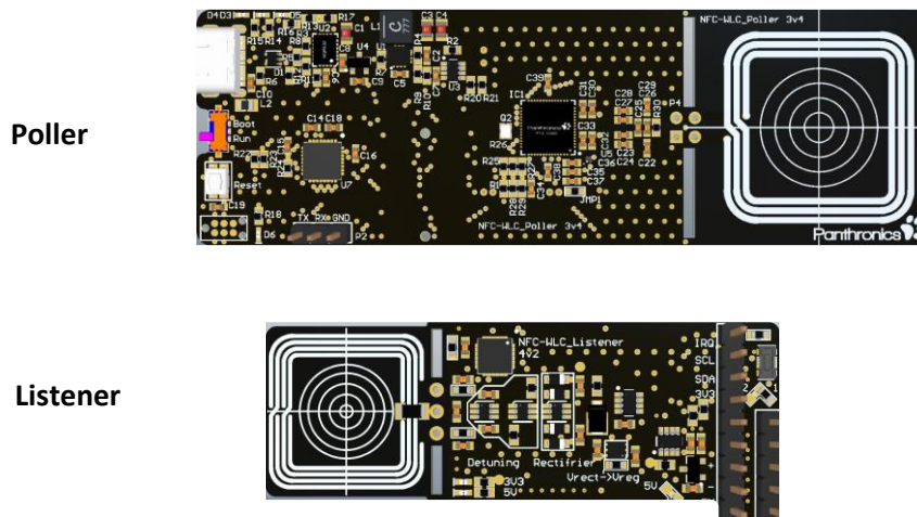
Fig. 3: Poller and Listener wireless charging boards used for WLC system demonstration (Image credit: Panthronics)
