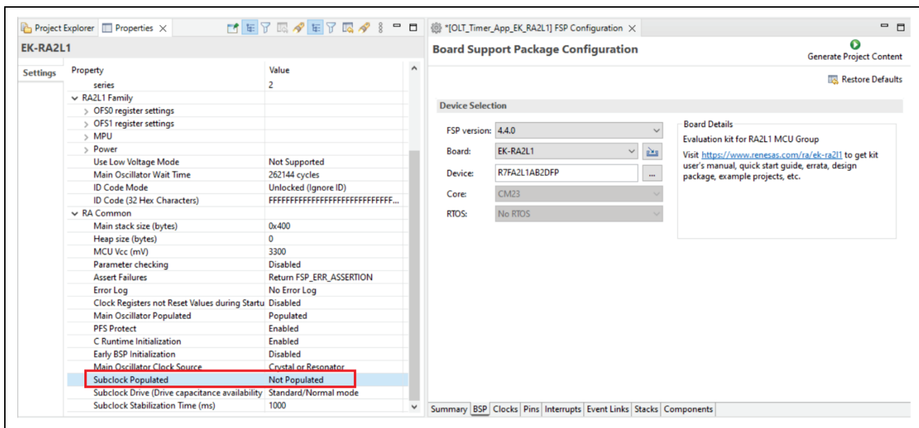
Figure 5. BSP Settings of the Operable Long Timer
