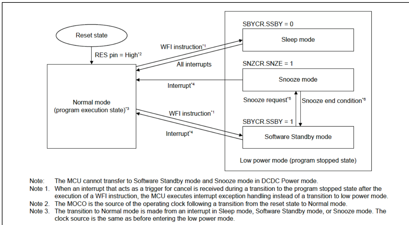
Figure 1. LPM Transition Diagram for RA2L1
