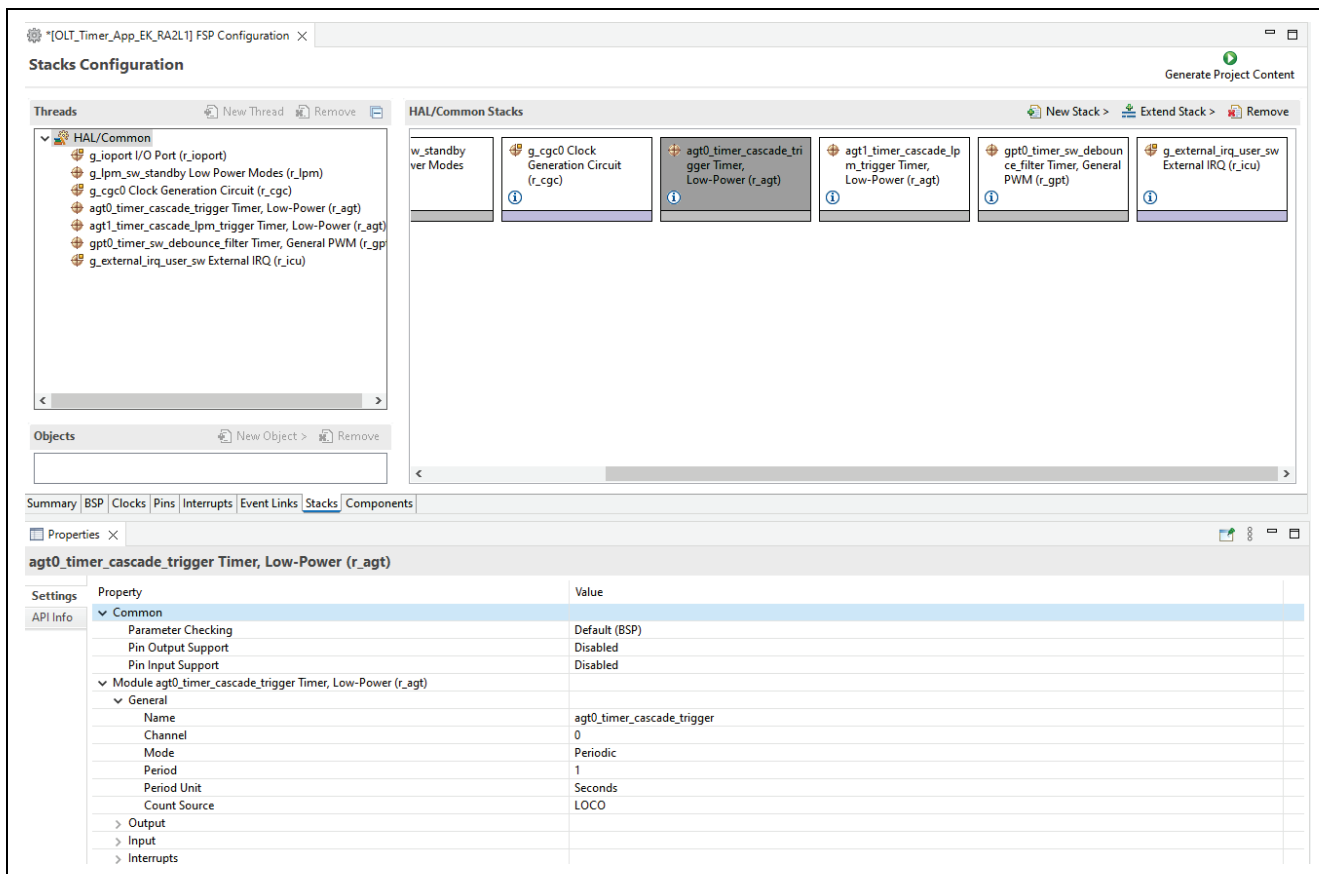
Figure 12. AGT0 Properties Configuration using the Properties Tab
