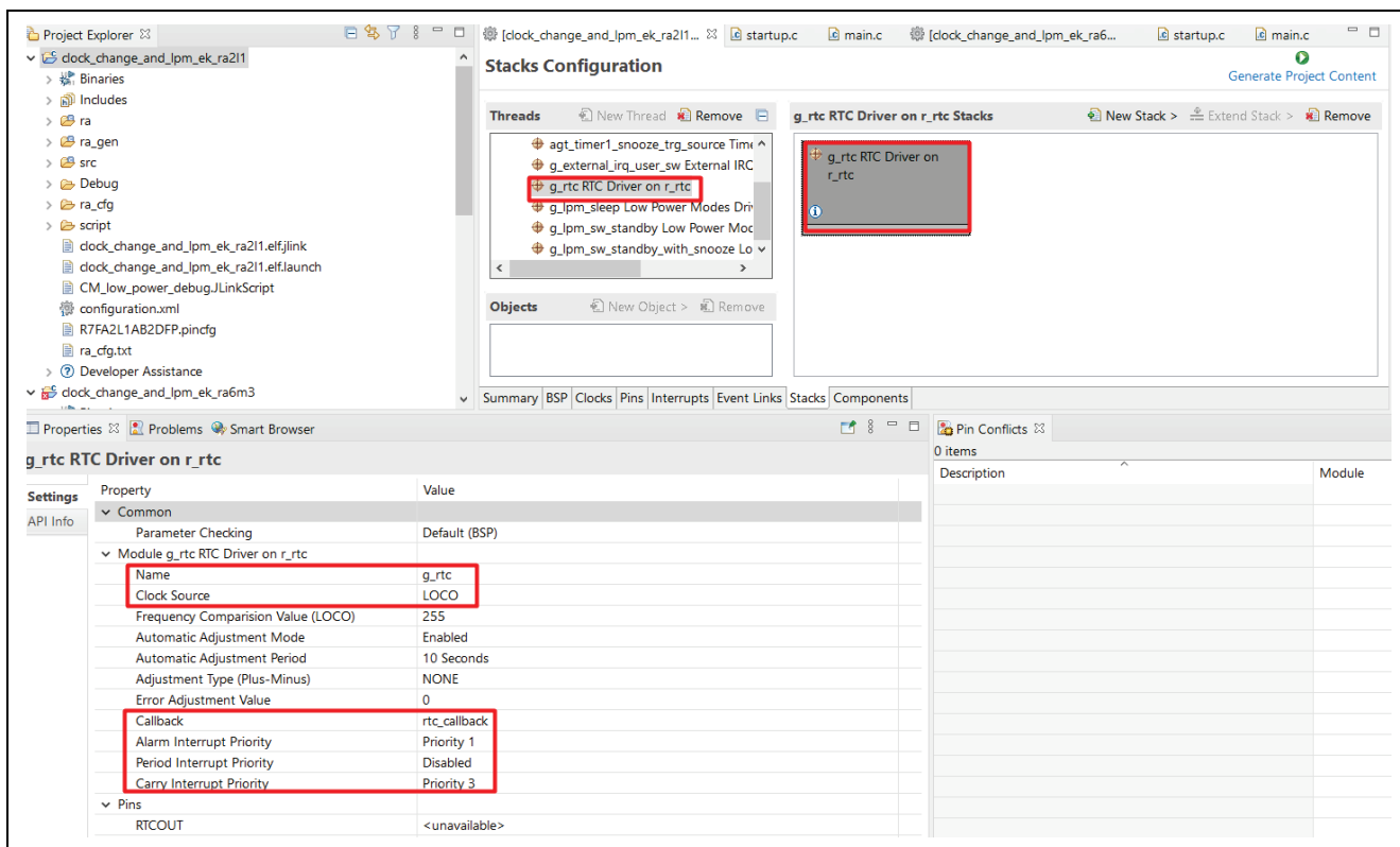
Figure 11. RTC Properties Configuration using the Properties Tab
