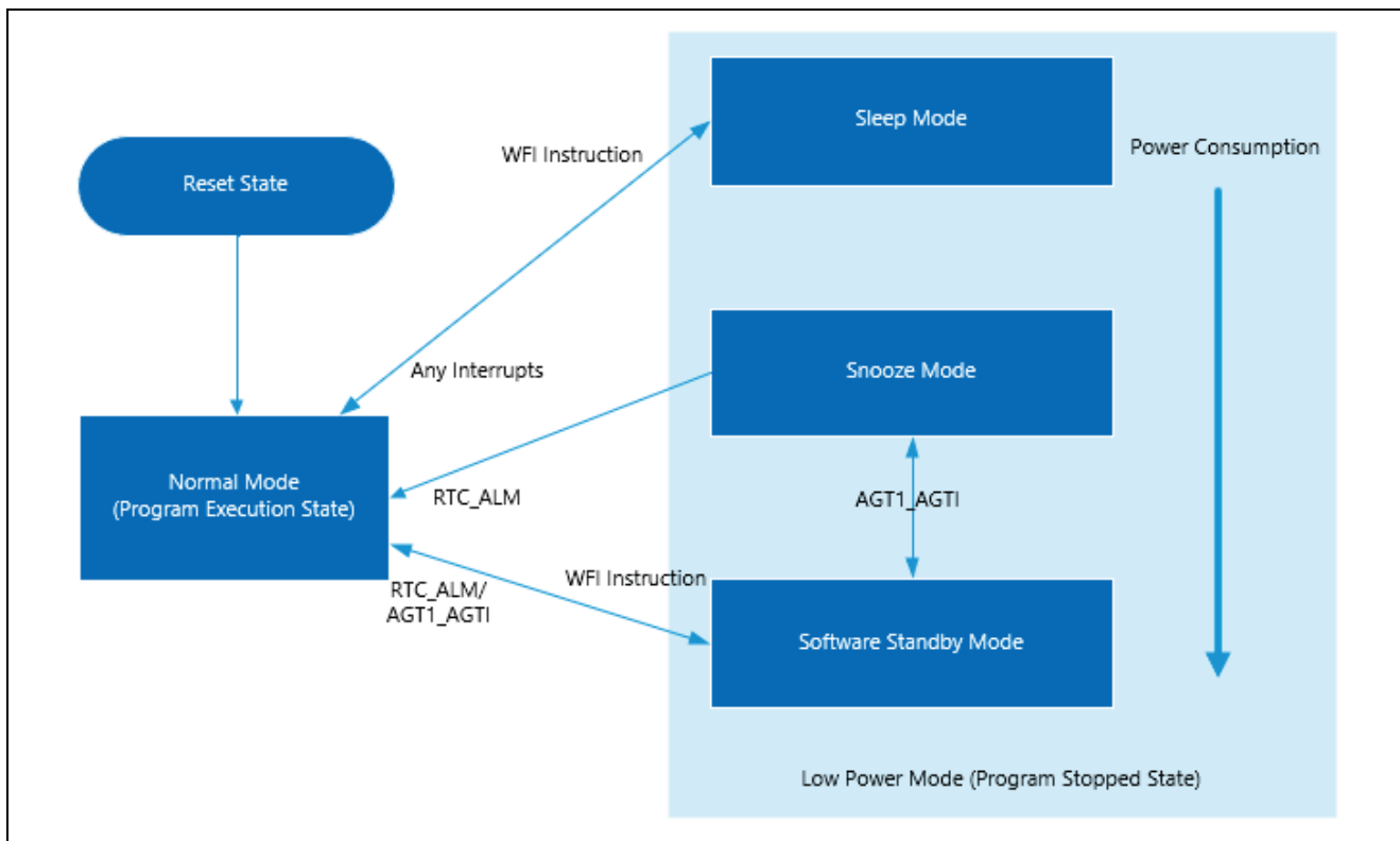
Figure 16. Transition Between LPM and Normal Mode
