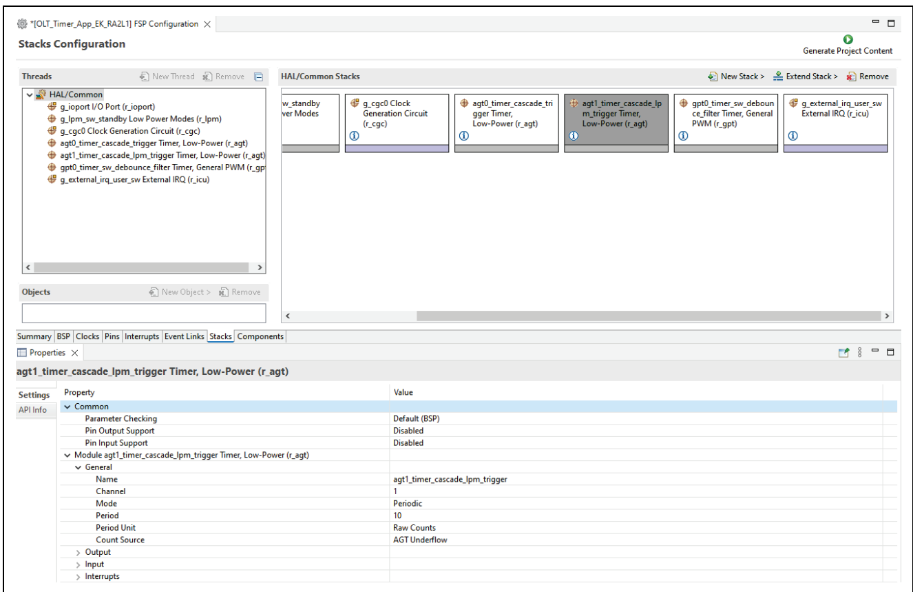
Figure 13. AGT1 Properties Configuration using the Properties Tab
