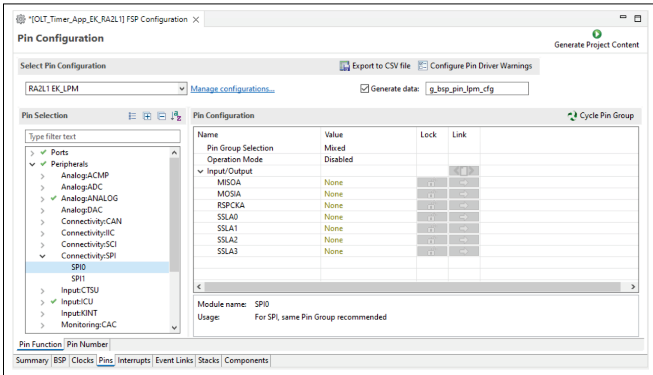
Figure 15. Pin Configuration of EK-RA2L1 Kit, Operating in LPM
