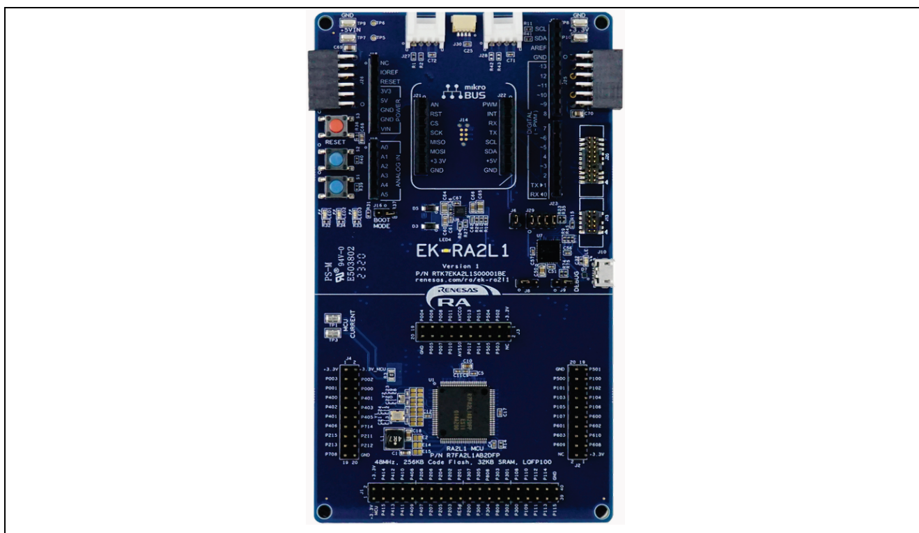
Figure 26. EK-RA2L1 Kit
