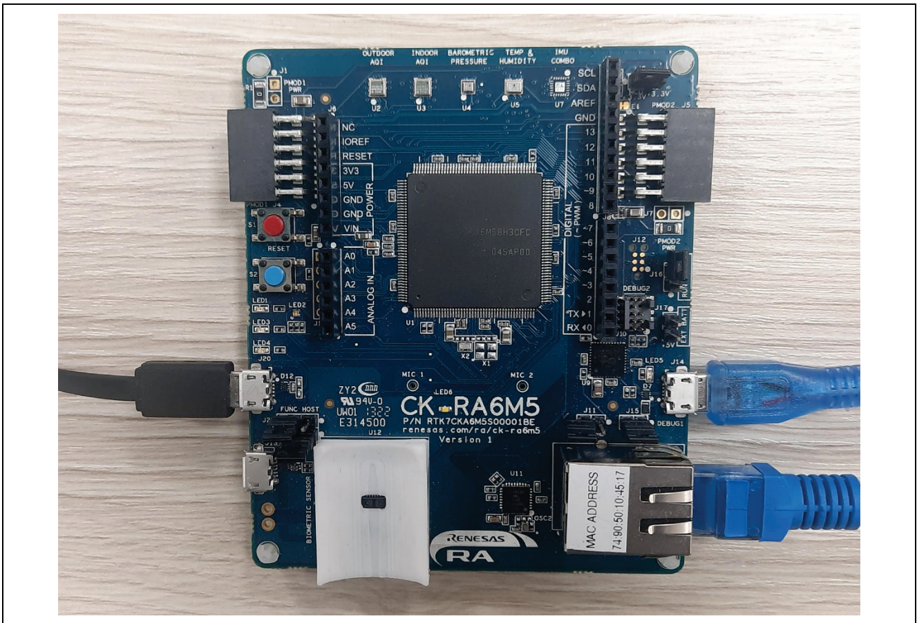
Figure 7. Hardware Setup
