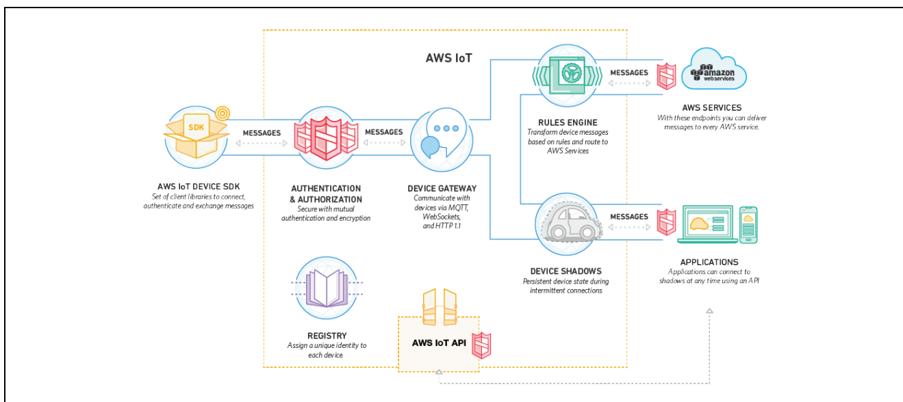
Figure 1. AWS IoT Features, Service Components, and Data Flow Diagram
