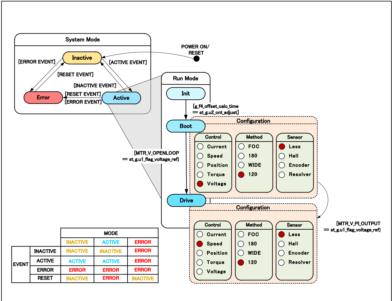
Figure 3-5 State Transition Diagram of Sensorless 120-degree Conducting Control Software
