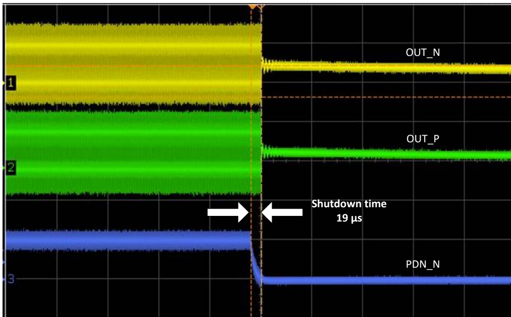
Figure 10. Shutdown timing (19 μs from de-asserting PDN_N to zero output)
