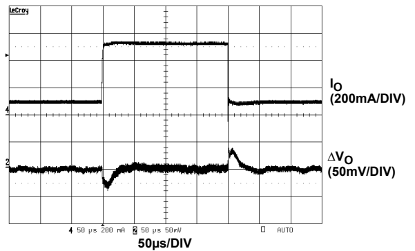
FIGURE 10. TRANSIENT RESPONSE (100mA to 500mA)
