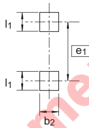
Pattern of terminal position areas
