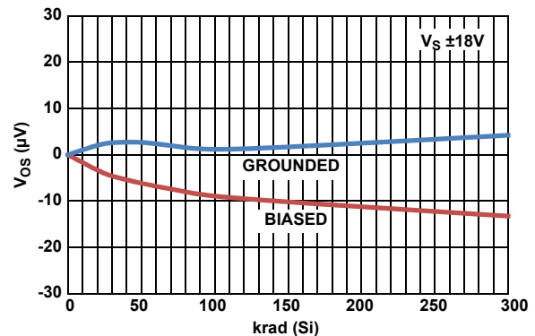
FIGURE 2. V_{0S} SHIFT vs HIGH DOSE RATE RADIATION
