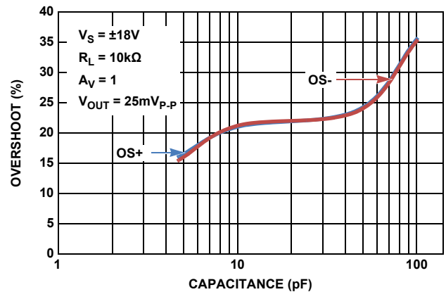
FIGURE 50. OVERSHOOT (%) vs LOAD CAPACITANCE
