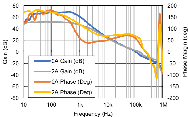
Figure 45. Ext Comp Gain/Phase BODE Plot, 3.3V IN , 1.0V OUT , 1MHz, R SLOPE = 34.8kΩ, R COMP = 14kΩ, C COMP = 1200pF, L OUT = 0.82μH, C OUT = 172μF
