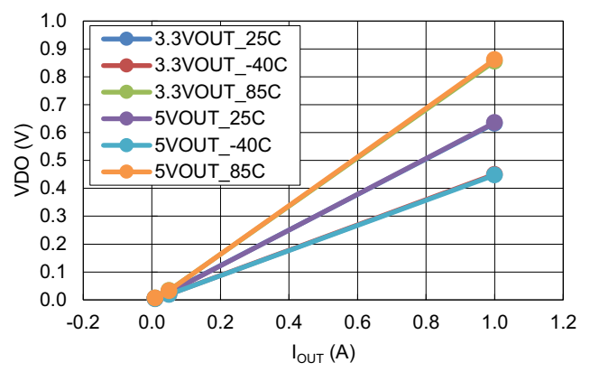
Figure 12. Dropout Voltage vs Output Current for Various Ambient Temperatures ( V_{OUT} = 3.3V and 5V ) SOIC Package
