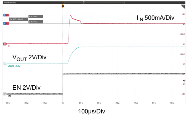
Figure 14. Startup and In-Rush Current for 25°C ( V_{IN} = 4.3V , V_{OUT} = 3.3V , C_{OUT} = 10\mu F , C_{FF} = 22pF , I_{OUT} = 1A )
