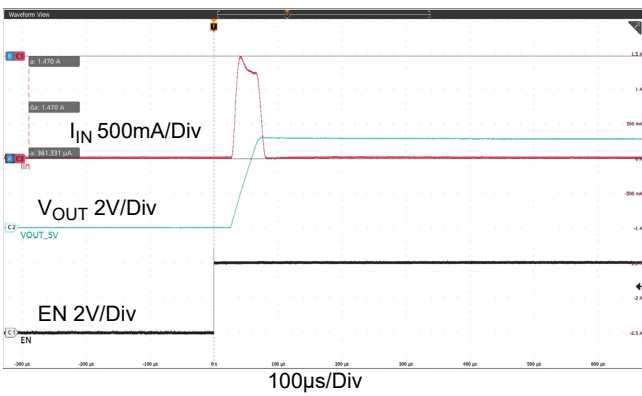
Figure 15. Startup and In-Rush Current for 25°C ( V_{IN} = 6V , V_{OUT} = 5V , C_{OUT} = 10\mu F , C_{FF} = 22pF , I_{OUT} = 0A )
