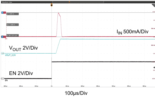
Figure 13. Startup and In-Rush Current for 25°C ( V_{IN} = 4.3V , V_{OUT} = 3.3V , C_{OUT} = 10\mu F , C_{FF} = 22pF , I_{OUT} = 0A )
