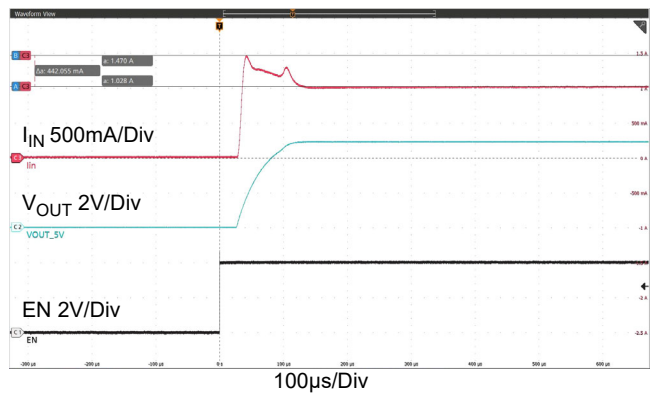
Figure 16. Startup and In-Rush Current for 25°C ( V_{IN} = 6V , V_{OUT} = 5V , C_{OUT} = 10\mu F , C_{FF} = 22pF , I_{OUT} = 1A )
