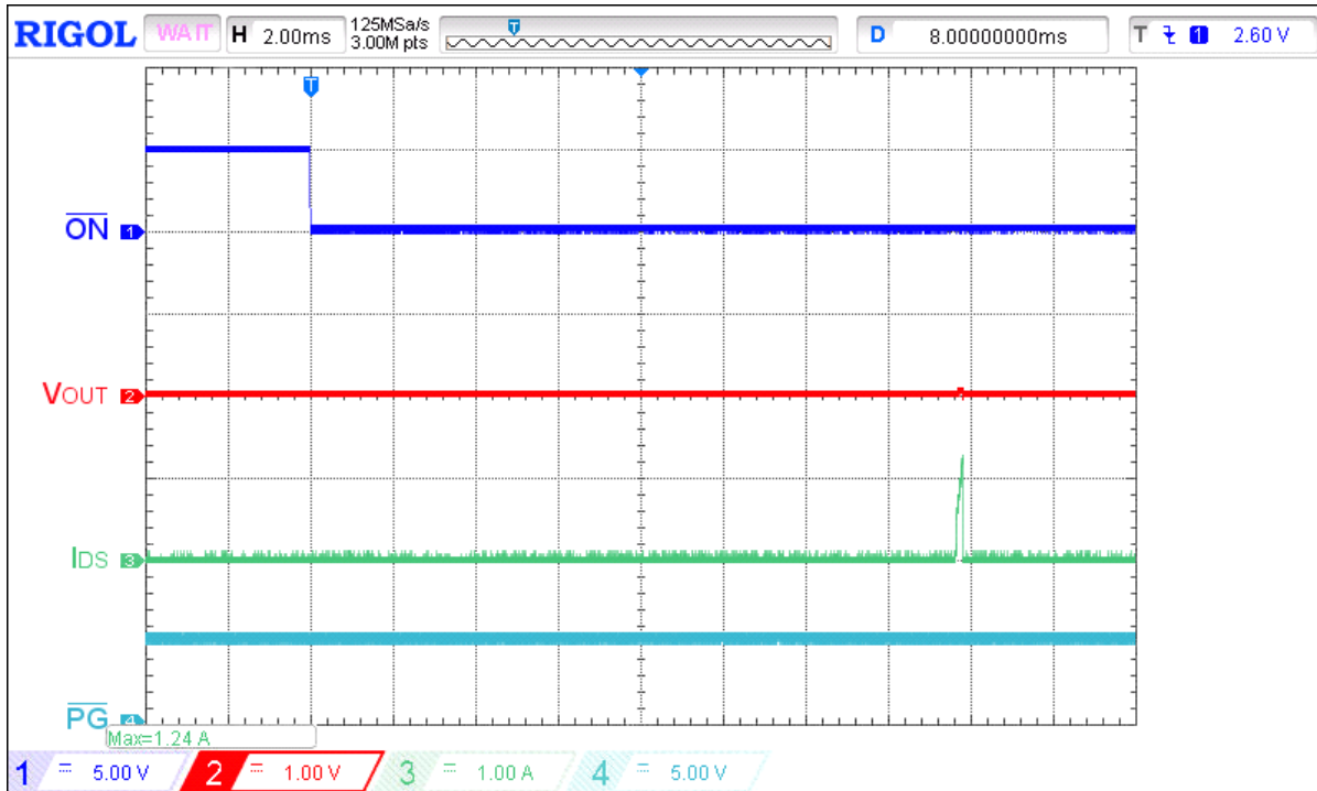
Figure 27. Startup Current Protection operation waveform for V_{\text{IN}} = 20 \text{ V} (extended view)
