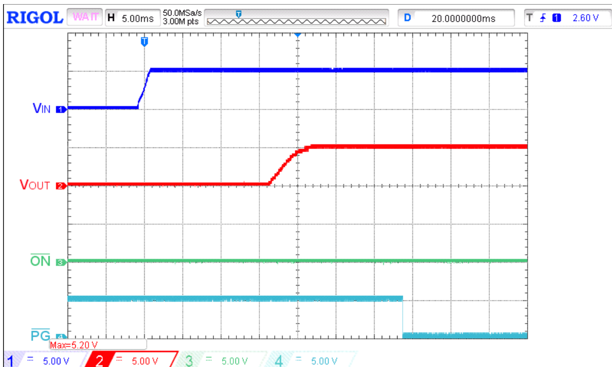
Figure 28. Typical Power Up operation waveform for V_{\text{IN}} = 5 \text{ V} , R_{\text{LOAD}} = 100 \Omega
