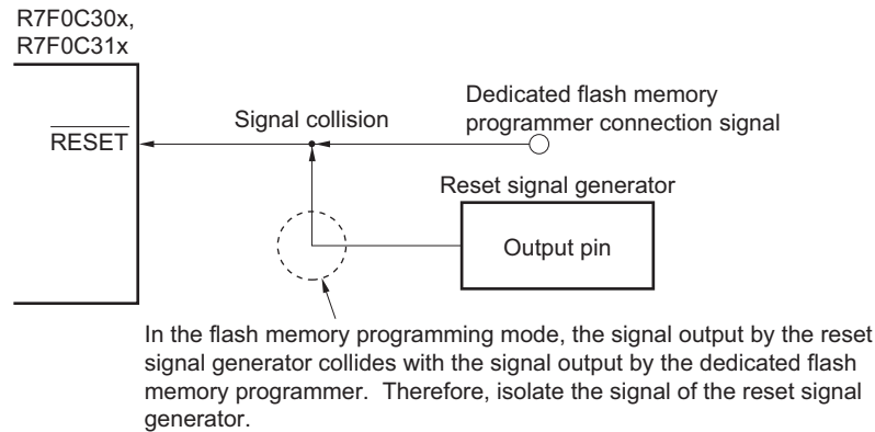
Figure 21-4. Signal Collision ( \overline{\text{RESET}} Pin)
