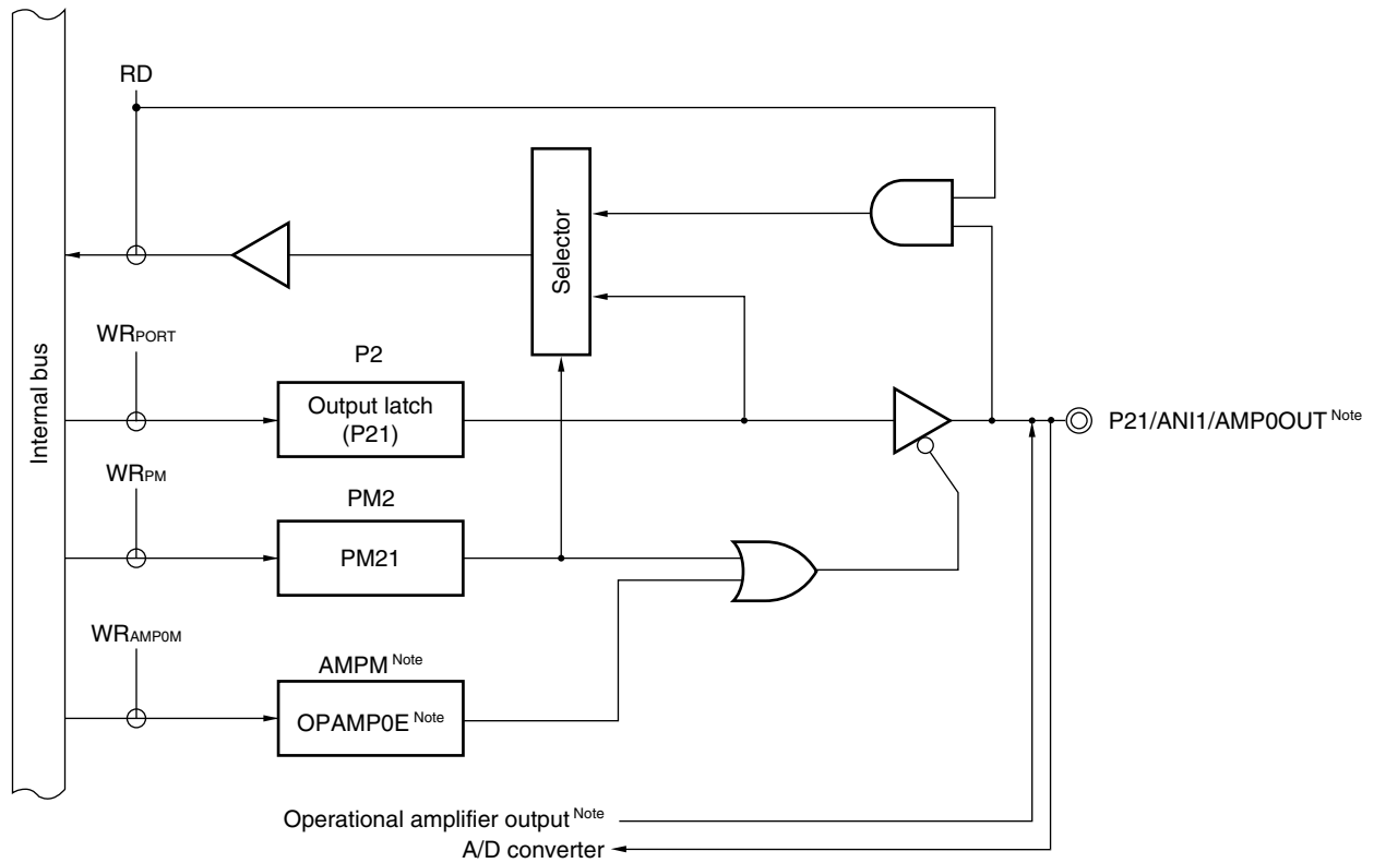
Figure 4-5. Block Diagram of P21
