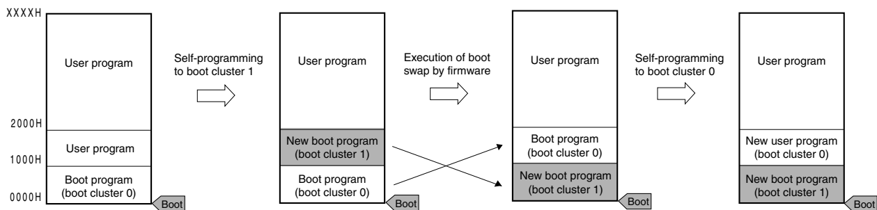
Figure 21-10. Boot Swap Function
