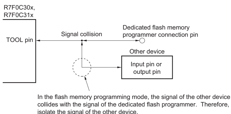
Figure 21-3. Signal Collision (TOOL Pin)
