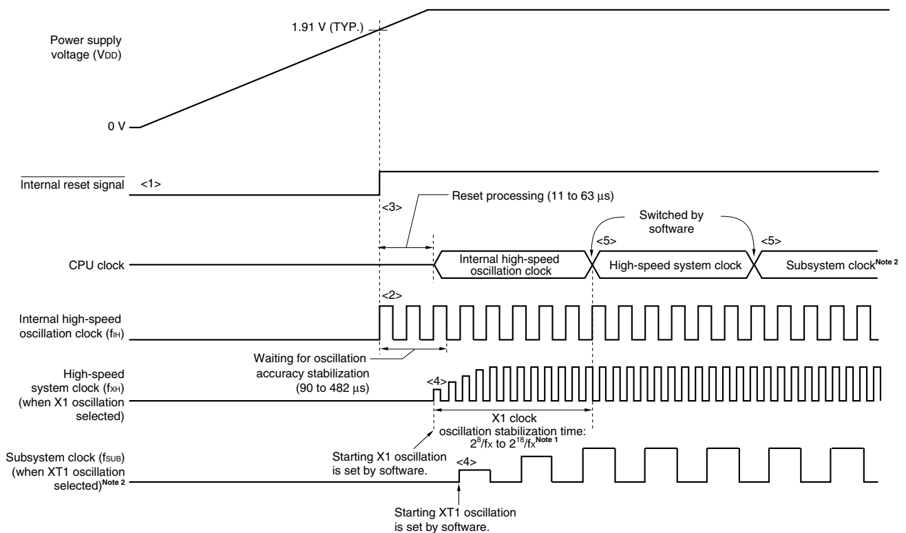
Figure 5-12. Clock Generator Operation When Power Supply Voltage Is Turned On (When LVI Default Start Function Enabled Is Set (Option Byte: LVISTART = 1))
