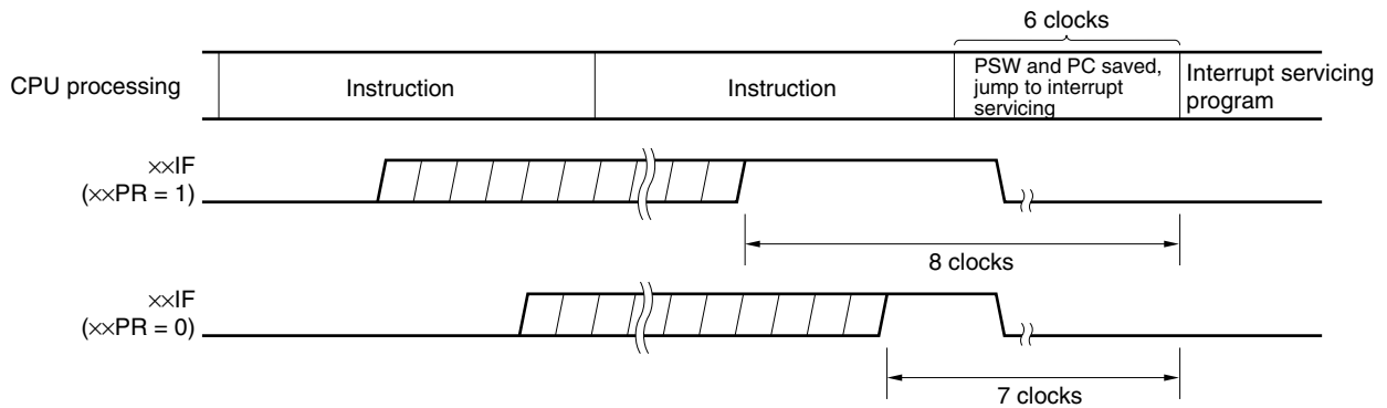
Figure 14-8. Interrupt Request Acknowledgment Timing (Minimum Time)
