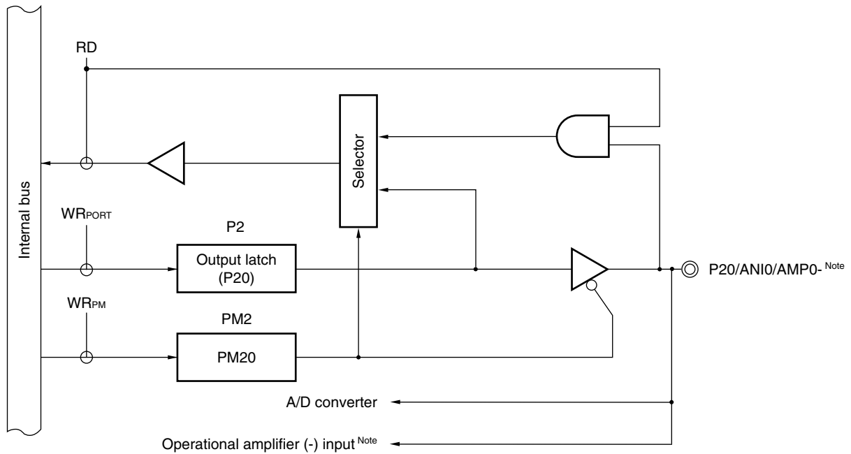
Figure 4-4. Block Diagram of P20
