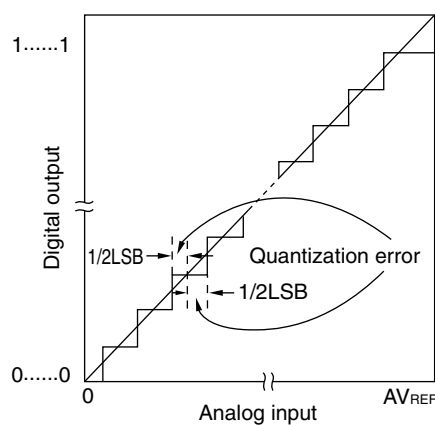
Figure 10-16. Quantization Error
