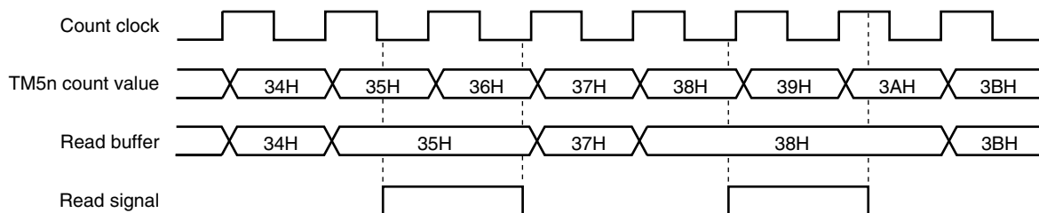
Figure 7-13. 8-bit Timer Counter 51 (TM51) Read Timing
