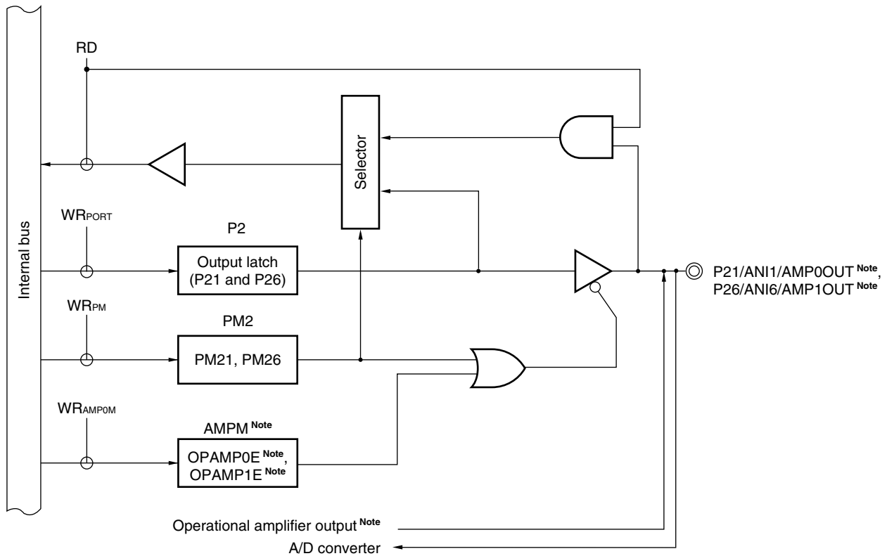
Figure 4-2. Block Diagram of P21 and P25
