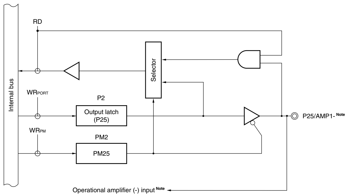
Figure 4-8. Block Diagram of P25
