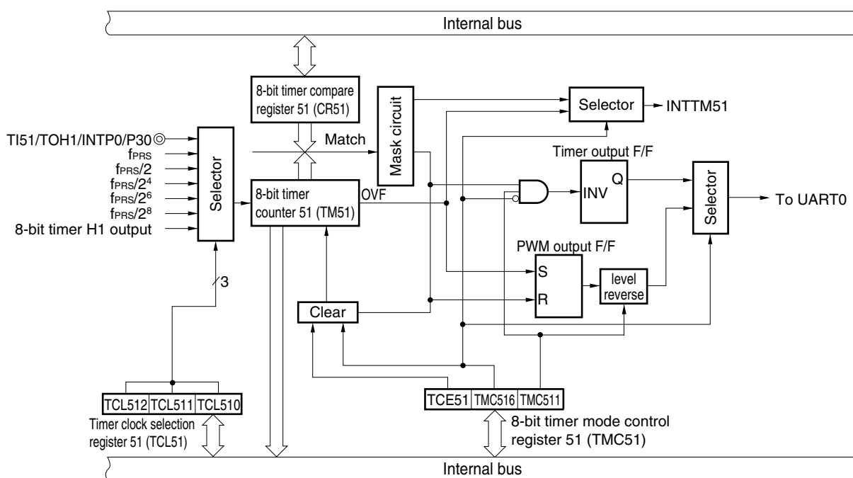
Figure 7-1. Block Diagram of 8-Bit Timer 51
