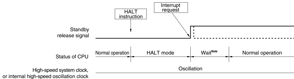
Figure 15-3. HALT Mode Release by Interrupt Request Generation
