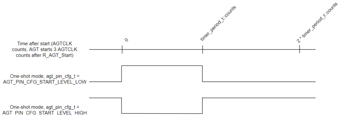
Figure 239: AGT One-Shot Output
