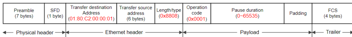
Figure 222: Pause Frame Format Image
