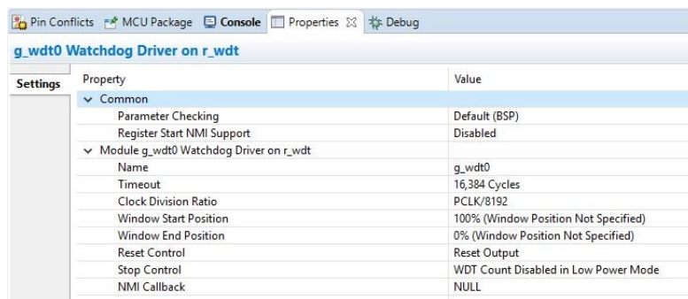
Figure 97: g_wdt WATCHDOG Driver on WDT properties
