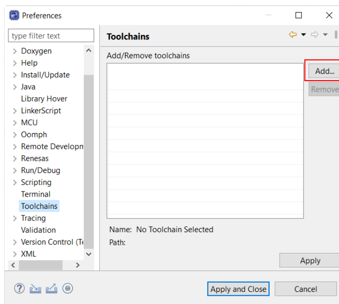
Figure 58: Add Toolchain
