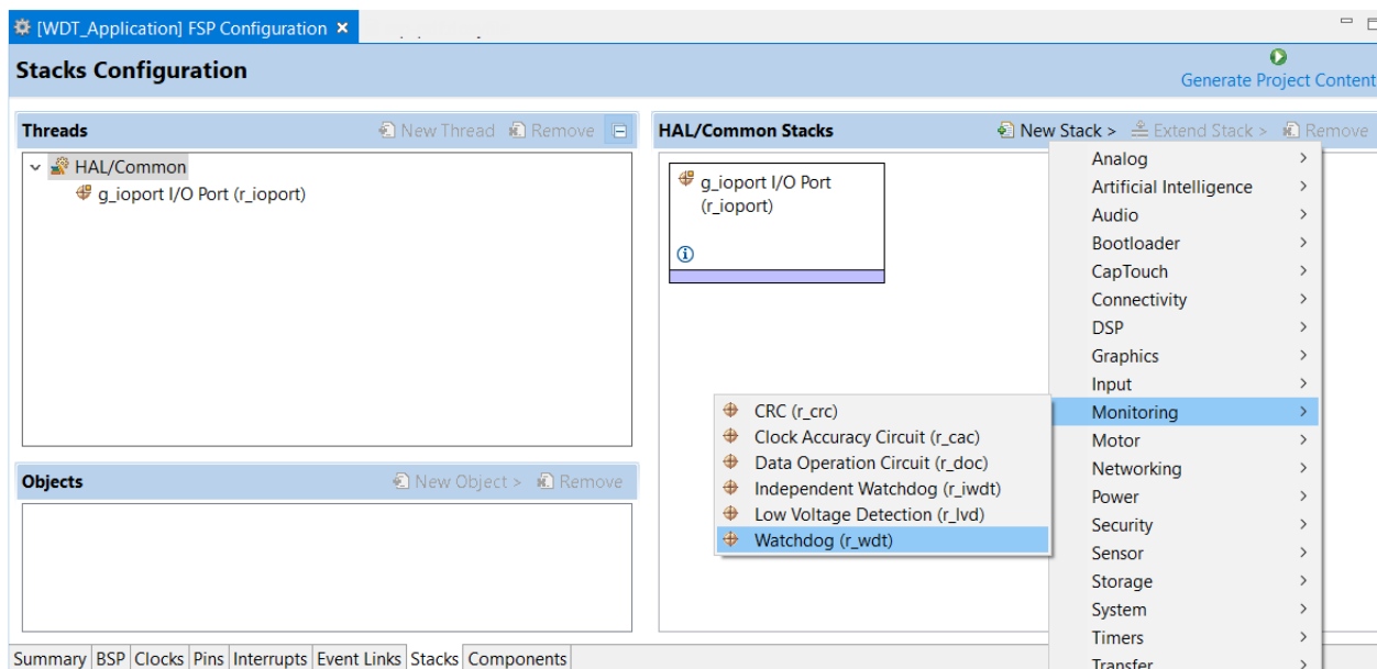
Figure 95: Module Selection
