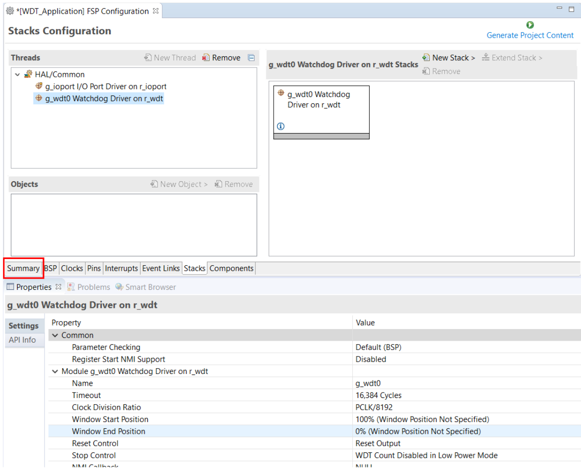
Figure 96: Module Properties
