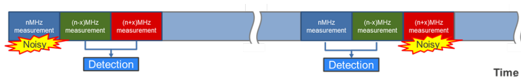
Figure 152: Multi-frequency Measurements
