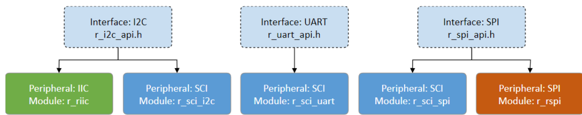
Figure 143: Instances
