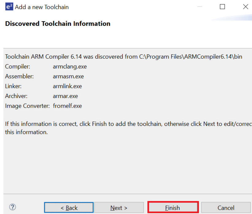
Figure 60: Toolchain Information
