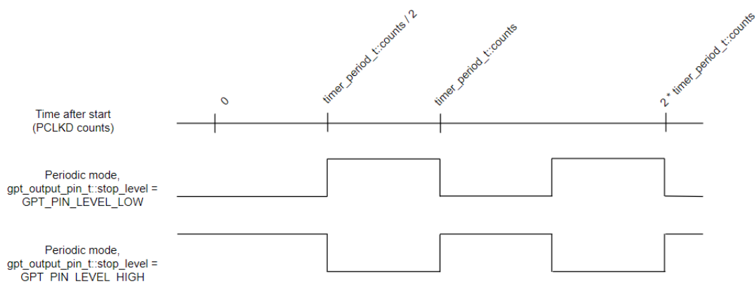
Figure 235: GPT Periodic Output
