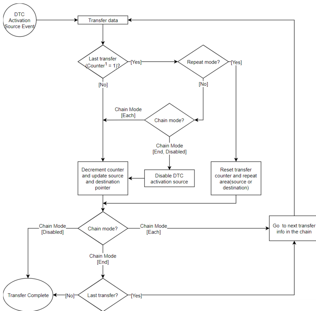
Figure 244: DTC Transfer Flowchart
