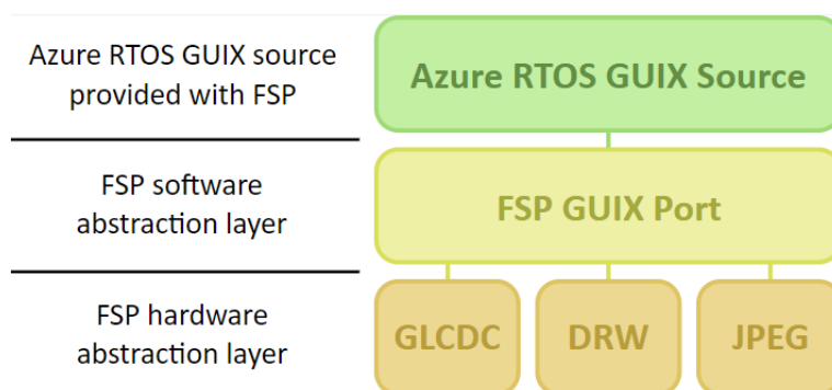
Figure 209: Azure RTOS GUIX Port Block Diagram
