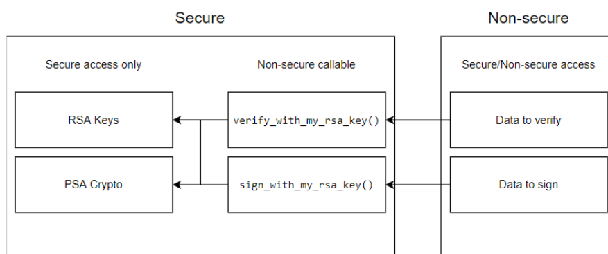
Figure 225: PSA Crypto Non-secure callable example
