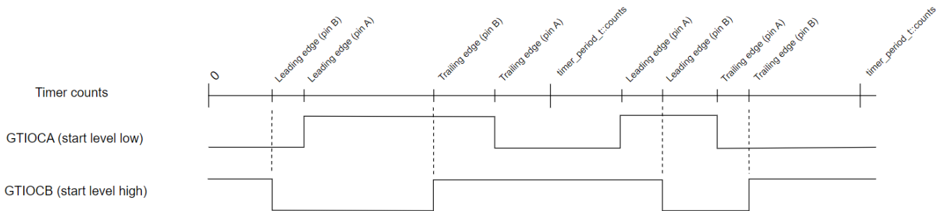
Figure 233: GPT One-Shot Pulse Output (without dead time)
