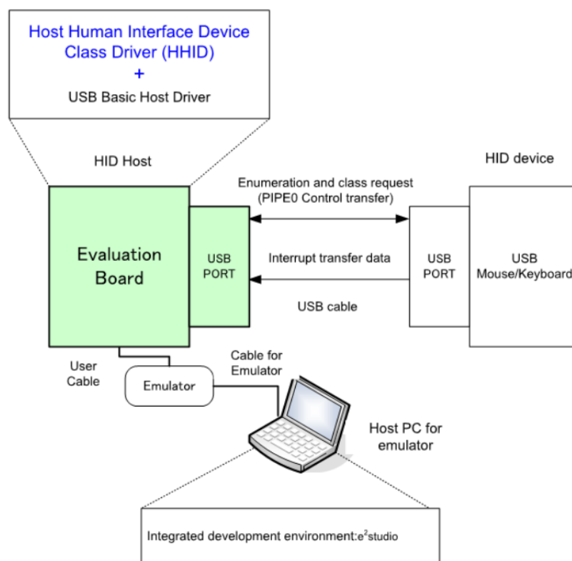
Figure 191: Example Operating Environment
