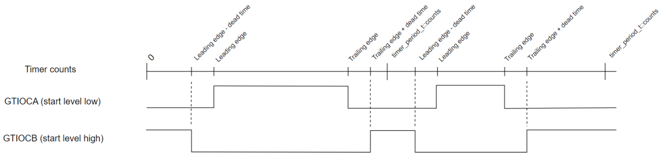
Figure 234: GPT One-Shot Pulse Output (with dead time)
