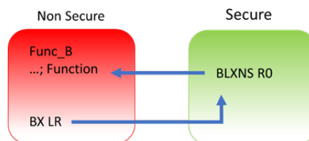
Figure 105: Calling from Secure to Non-Secure Functions
