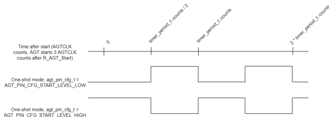
Figure 240: AGT Periodic Output
