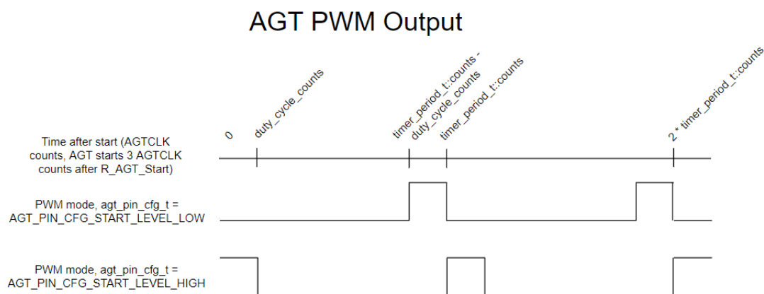
Figure 241: AGT PWM Output
