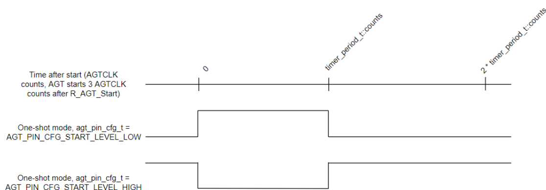
Figure 239: AGT One-Shot Output
