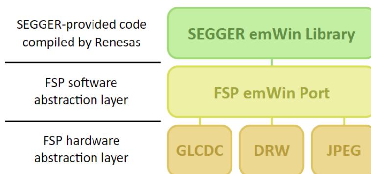
Figure 213: SEGGER emWin FSP Port Block Diagram
