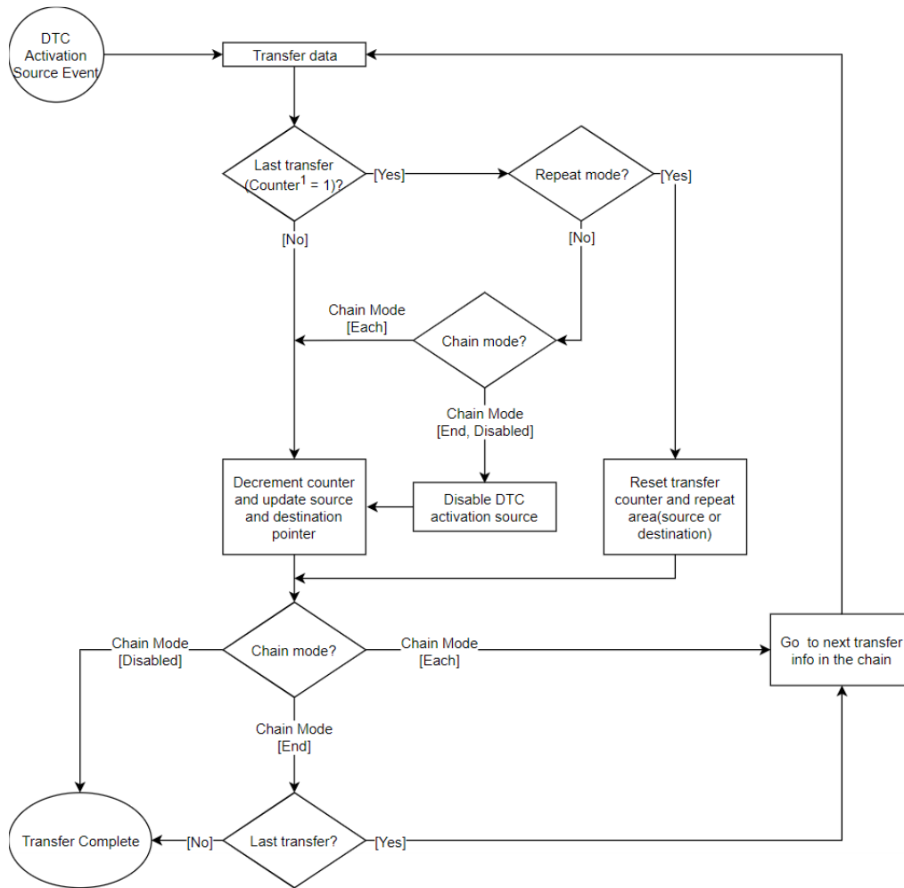
Figure 242: DTC Transfer Flowchart
