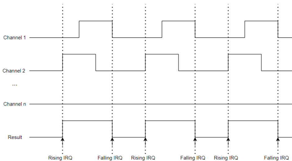
Figure 224: IPLS IRQ Generation
