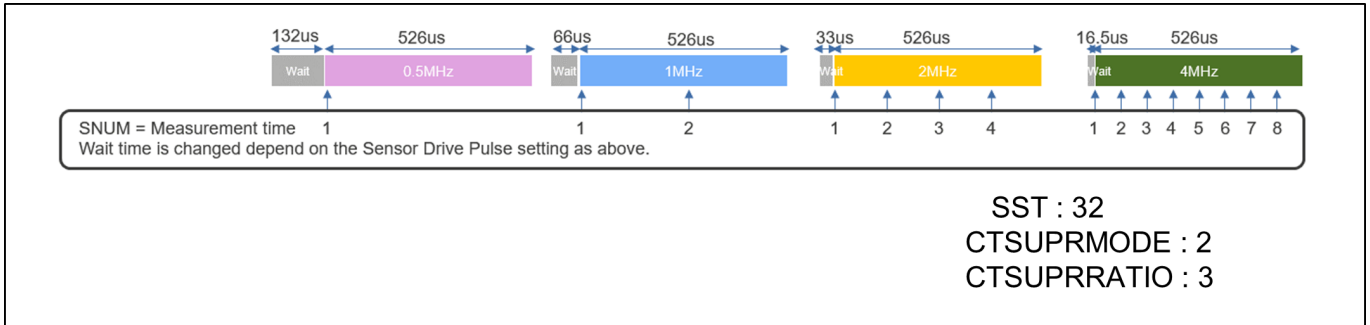
Figure 155: Self-capacitance Measurement Period (CTSU1)
