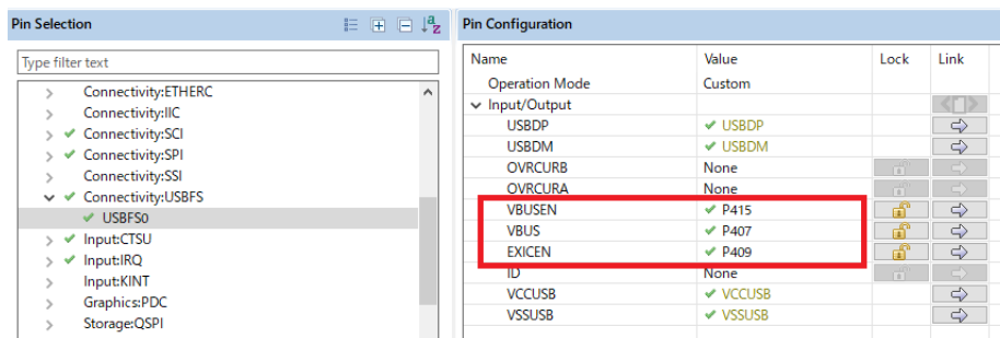
Figure 175: USB Pin Setting
