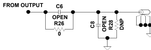
FIGURE 4. OUTPUT STAGE (1/2)
