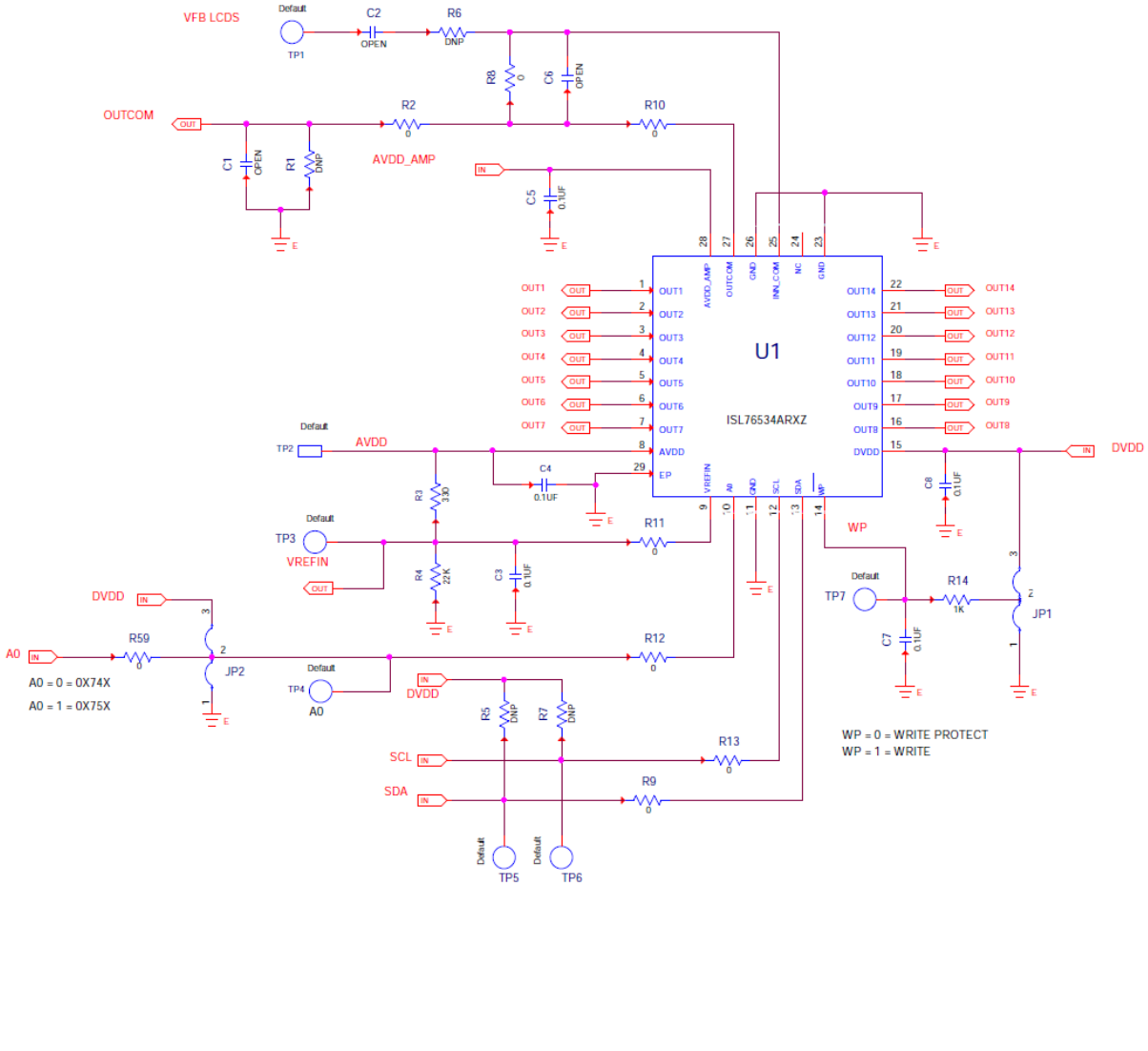
FIGURE 13. SCHEMATIC
