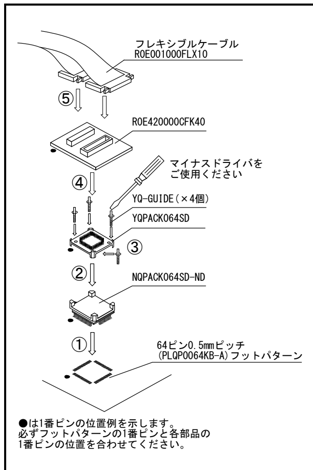
図3 ROE420000CFK40装着手順
