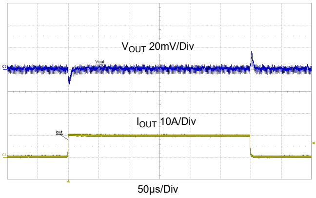
Figure 26. Transient Response, V_{IN} = 12V , V_{OUT} = 0.8V , 0A to 15A to 0A, 5A/\mu s Step Load, C_{OUT} = 10 \times 47\mu F Ceramic + 2 \times 470\mu F Polymer Capacitor
