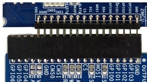
Figure 11. Dongle Connection
