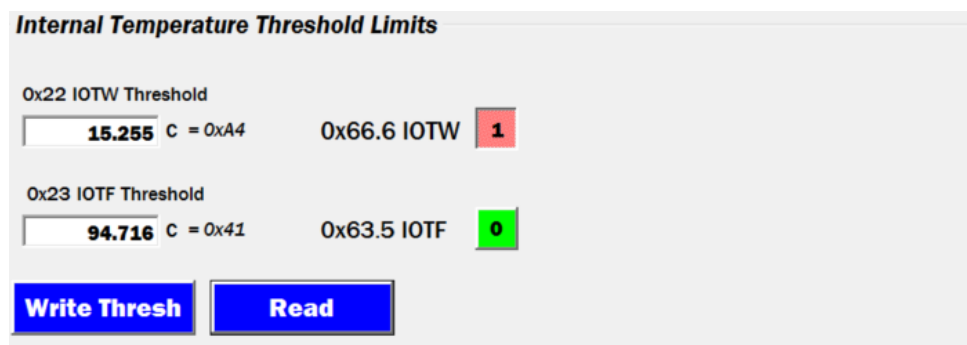
Figure 51. IOTW
