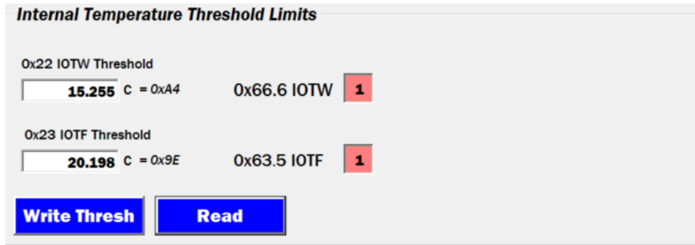
Figure 52. IOTF
