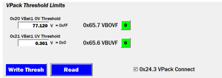
Figure 47. VBat1 OV
