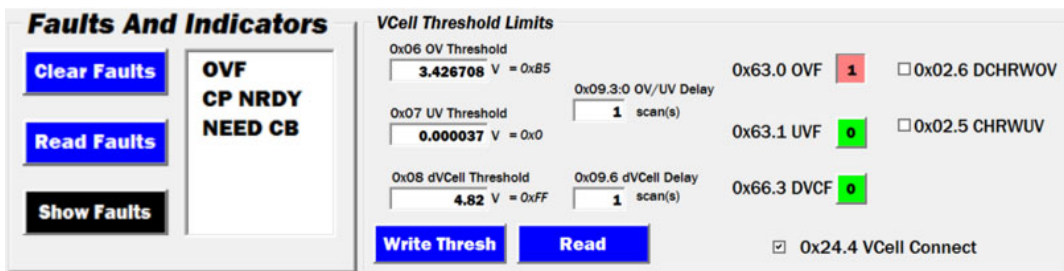
Figure 29. OV Fault
