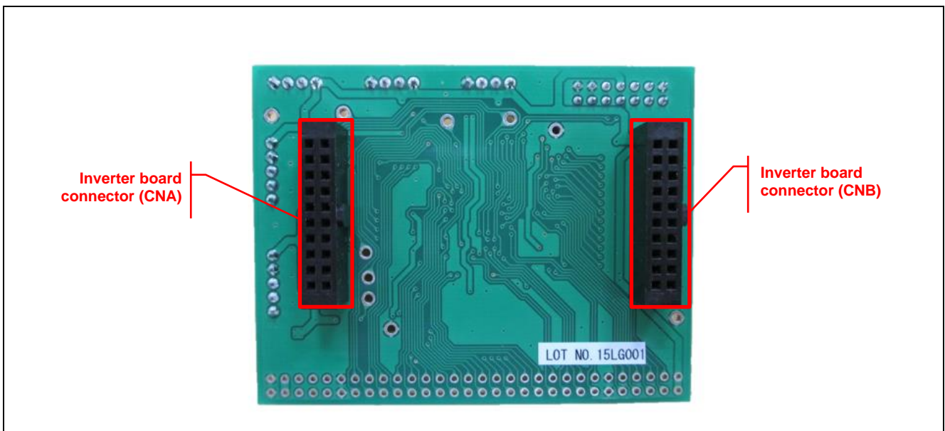
Figure 3.2 RX24T CPU Card Layout (Bottom view)
