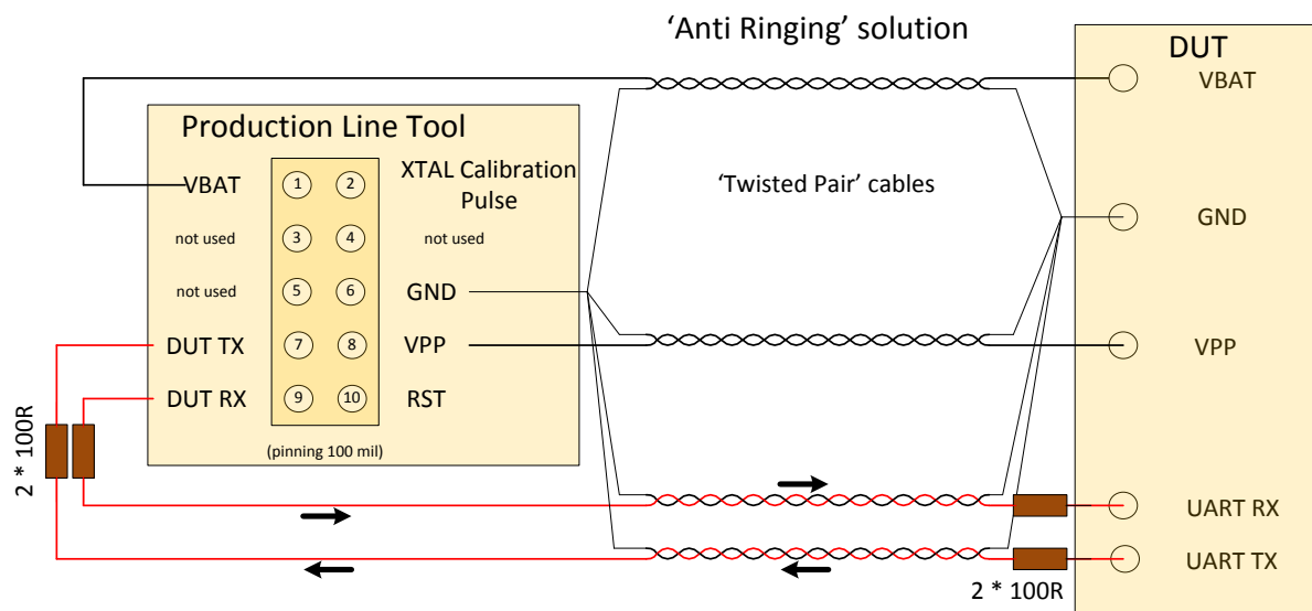
Figure 171: Anti-Ringing Solution
