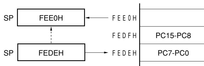
(c) RETI, RETB命令 (SPがFEDEHの場合)
