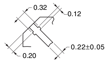
DETAIL OF (B) PART
