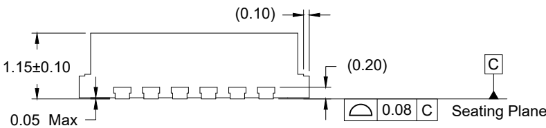
SIDE VIEW
