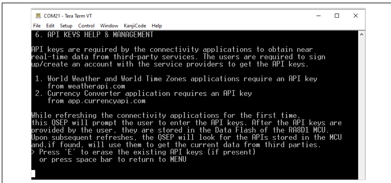
図 35. API Keys Help &amp; Management
