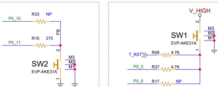
USER BUTTON
