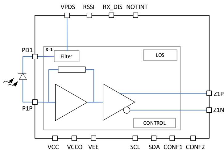
Figure 1. Block Diagram
