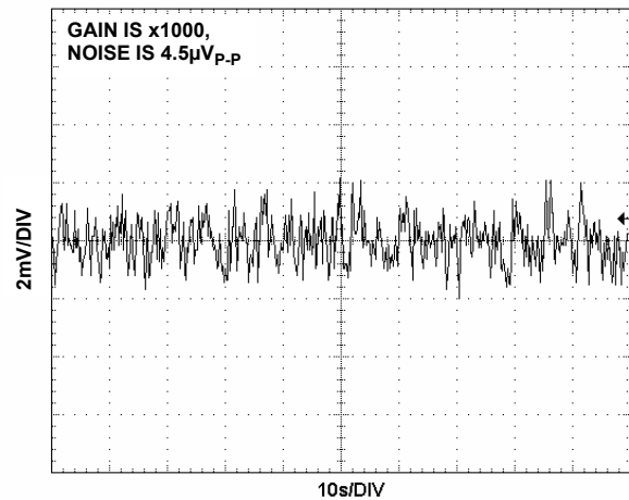
FIGURE 26. V_{OUT} NOISE, 0.1Hz TO 10Hz
