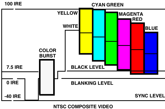
FIGURE 8. COMPOSITE VIDEO STANDARD
