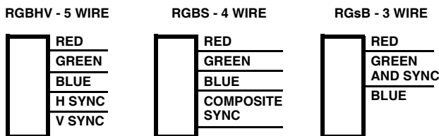
FIGURE 4. WIRES REQUIRED FOR RGBHV vs RGSB vs RGSB VIDEO
