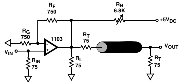
FIGURE 2. EL8102 APPLICATION CIRCUIT VIDEO AMPLIFIER WITH SYNC STRIPPER
