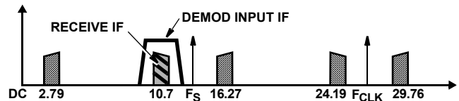
FIGURE 3. SAMPLED SPECTRUM FOR THE -27 VERSIONS ( f_{CLK} = 26.97\text{MHz} )
