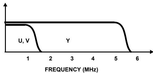
FIGURE 1C. Y-U, V SIGNAL BANDWIDTHS (PAL)
