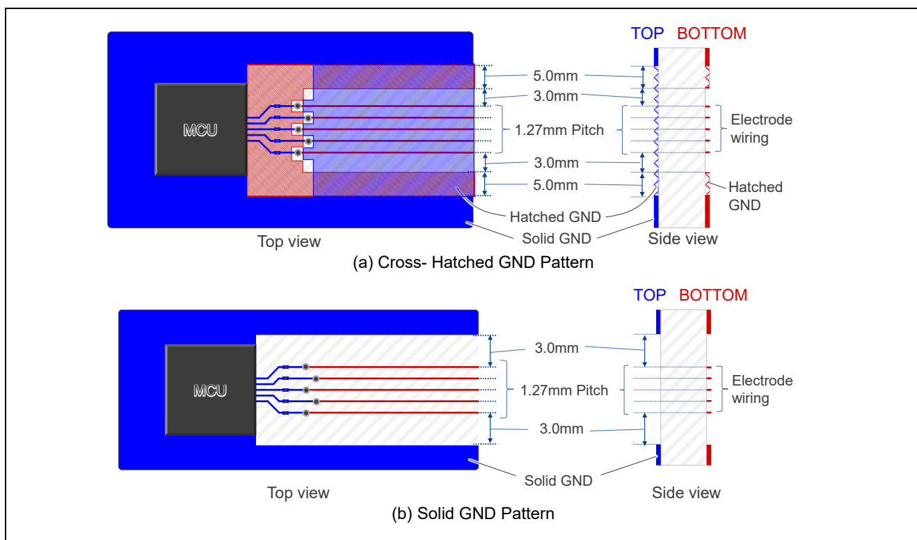
Figure2-9. Double-Layer Board Layout Example (wiring section)
