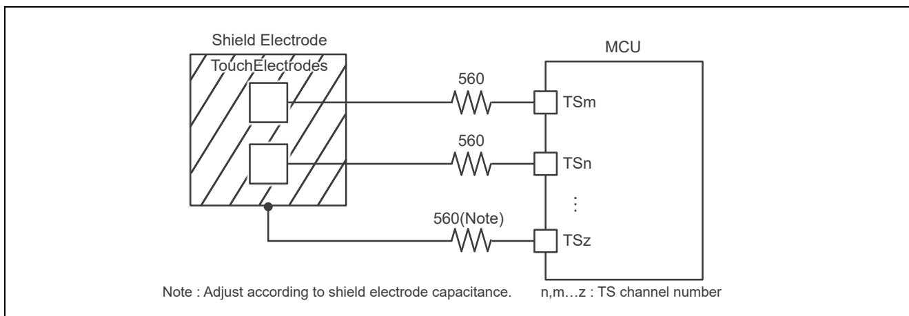
Figure2-17. Shield Electrode Circuit
