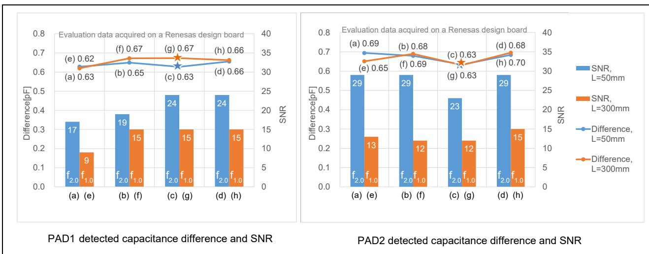
Figure 5-16 Wiring Pitch and Sensitivity Characteristics
