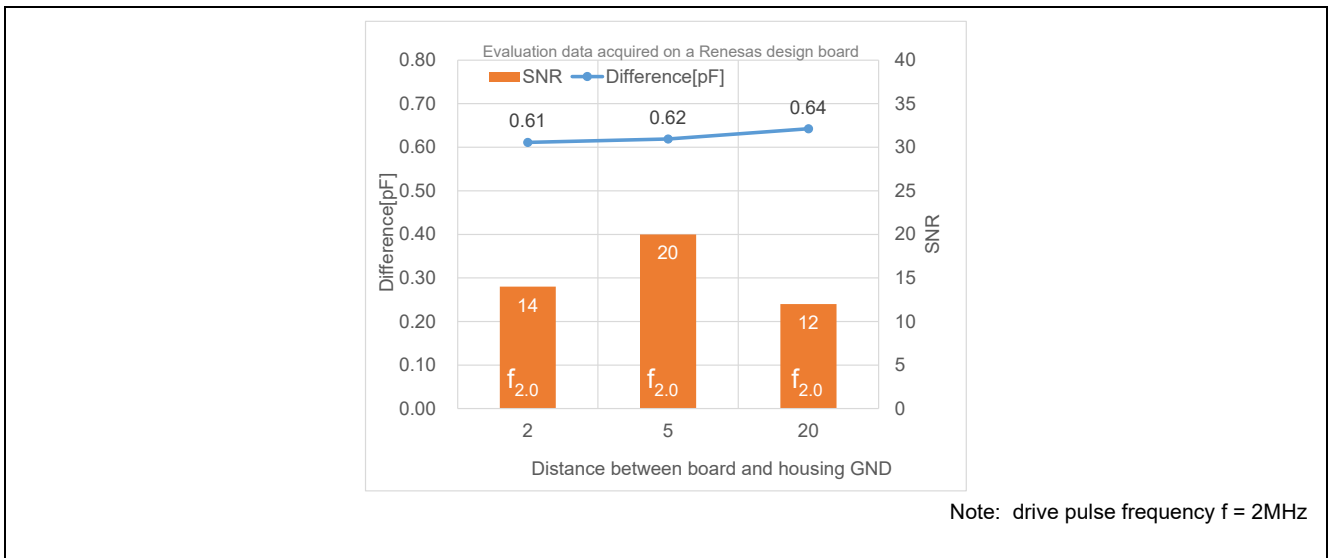
Figure 5-56 Board-Housing GND Distance and Sensitivity Characteristics
