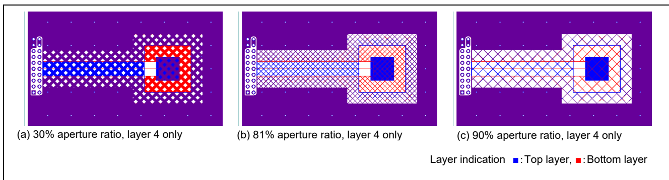
Figure 5-33 Evaluation Board Patterns (double-sided board, GND shield)
