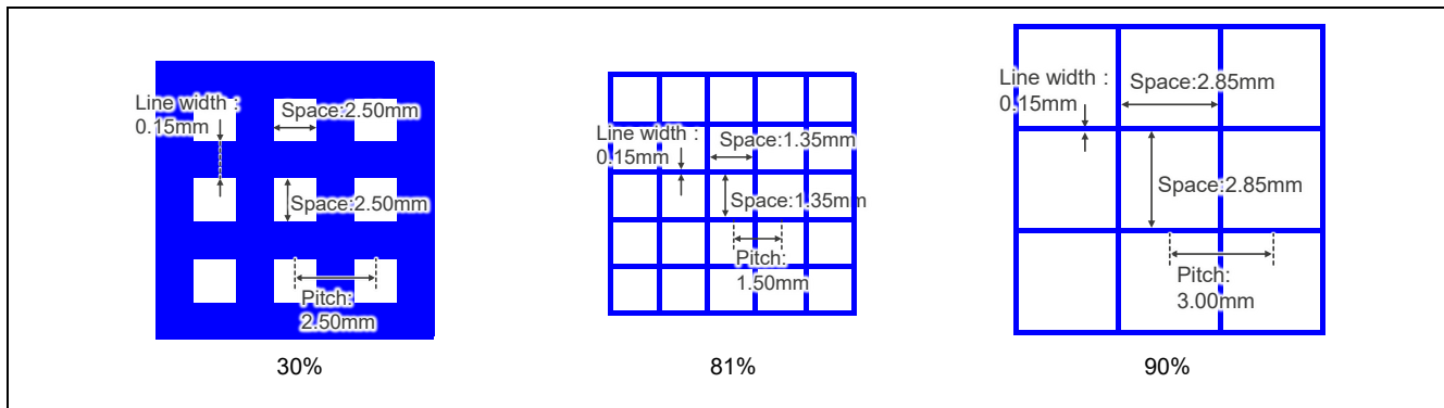
Figure 5-32 Cross-hatched Pattern Dimensions
