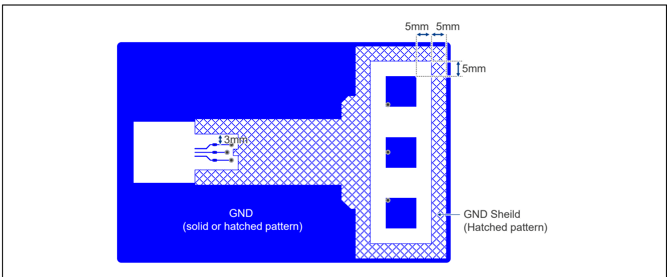
Figure2-15. GND Shield Pattern Example for Multi-layer Board (top layer)
