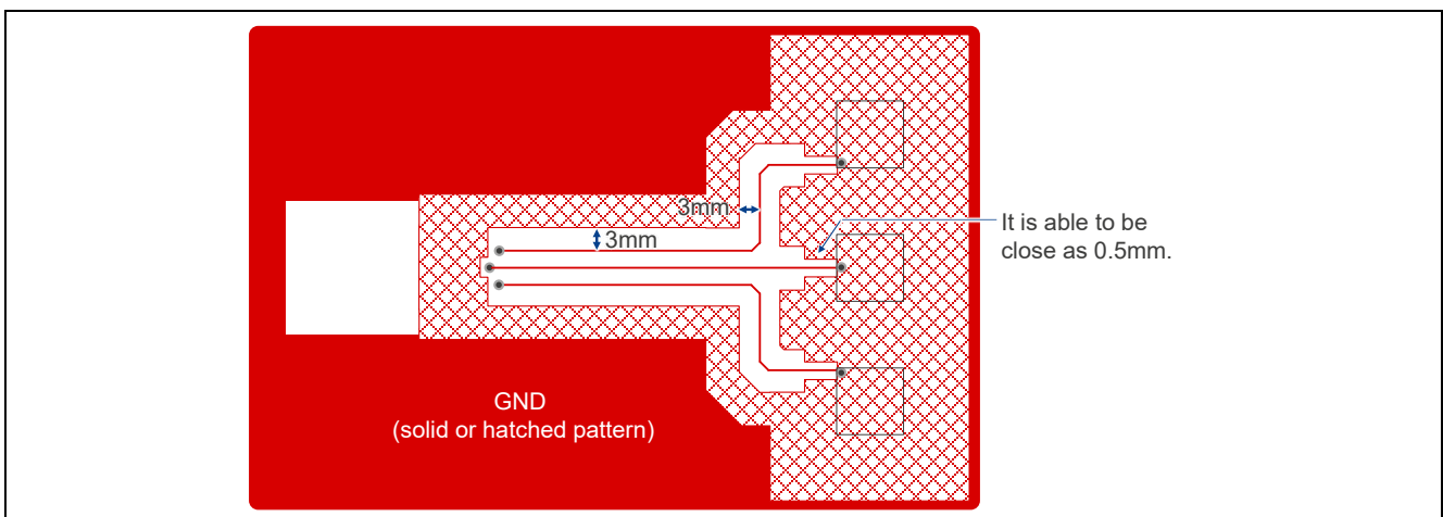
Figure2-16. GND Shield Pattern Example for Multi-layer Board (bottom layer)
