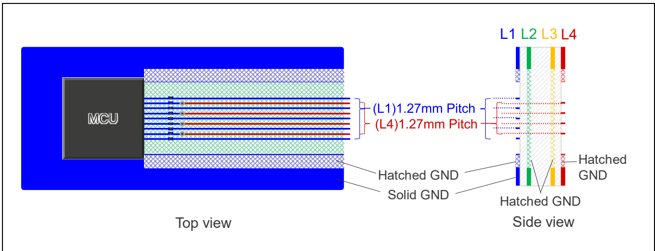
Figure2-13. High-density Wiring
