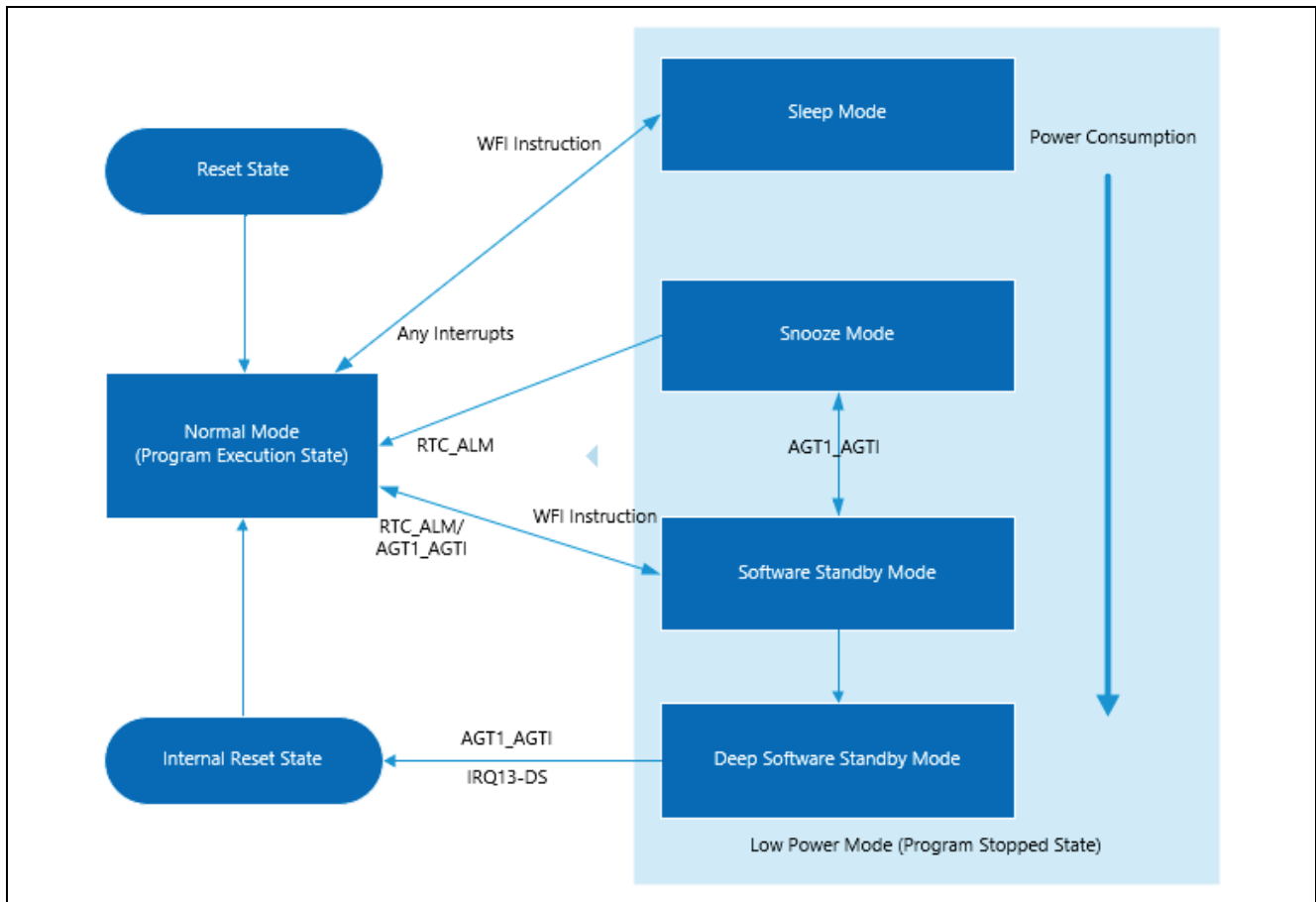
Figure 18. Transition Between LPM and Normal Mode
