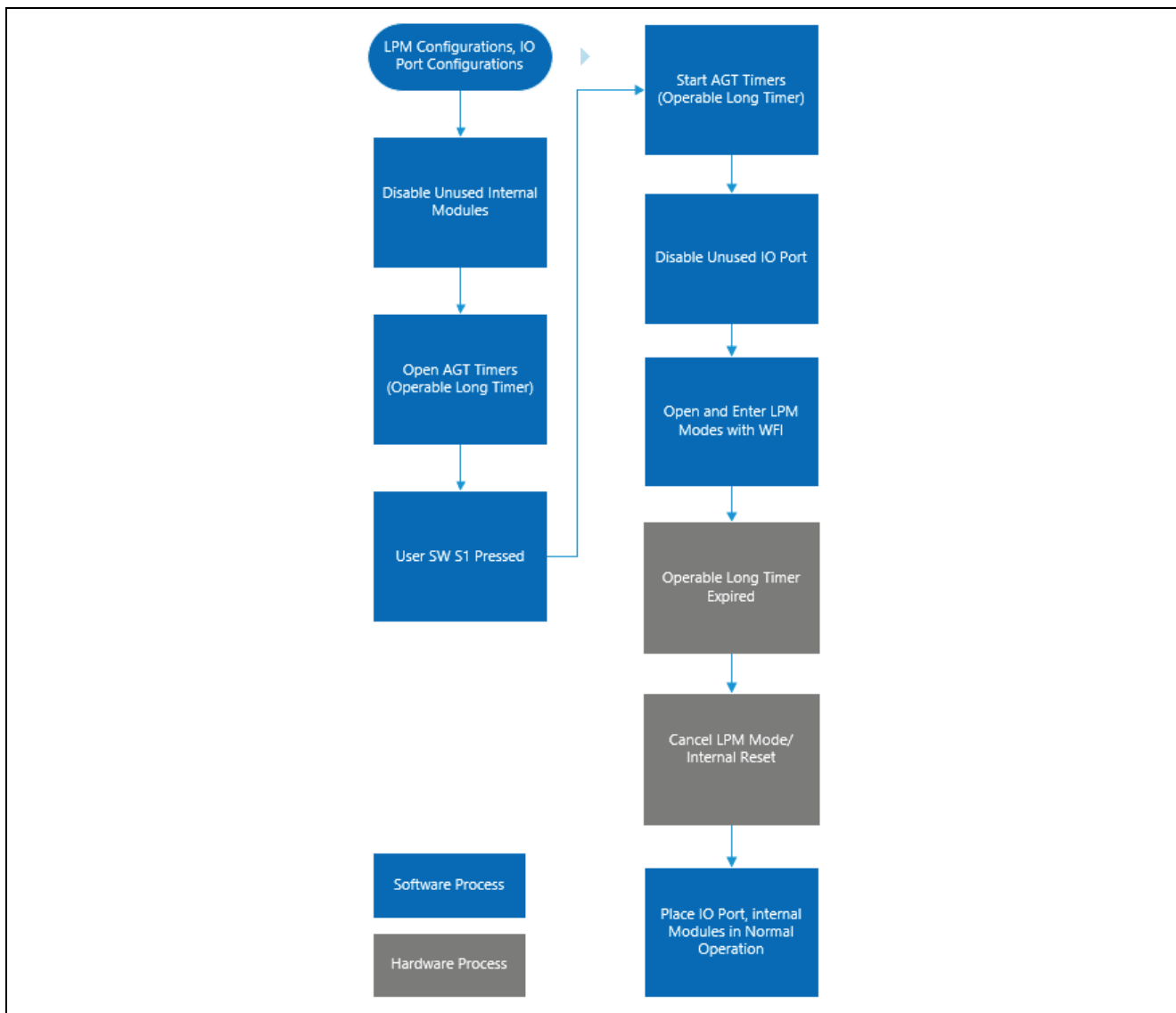
Figure 20. Operable Long Timer Process
