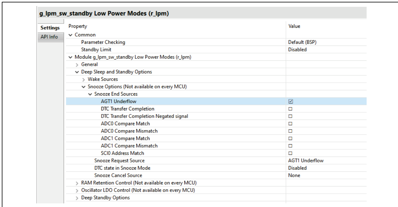
Figure 10. Snooze Properties Configuration using the Properties Tab
