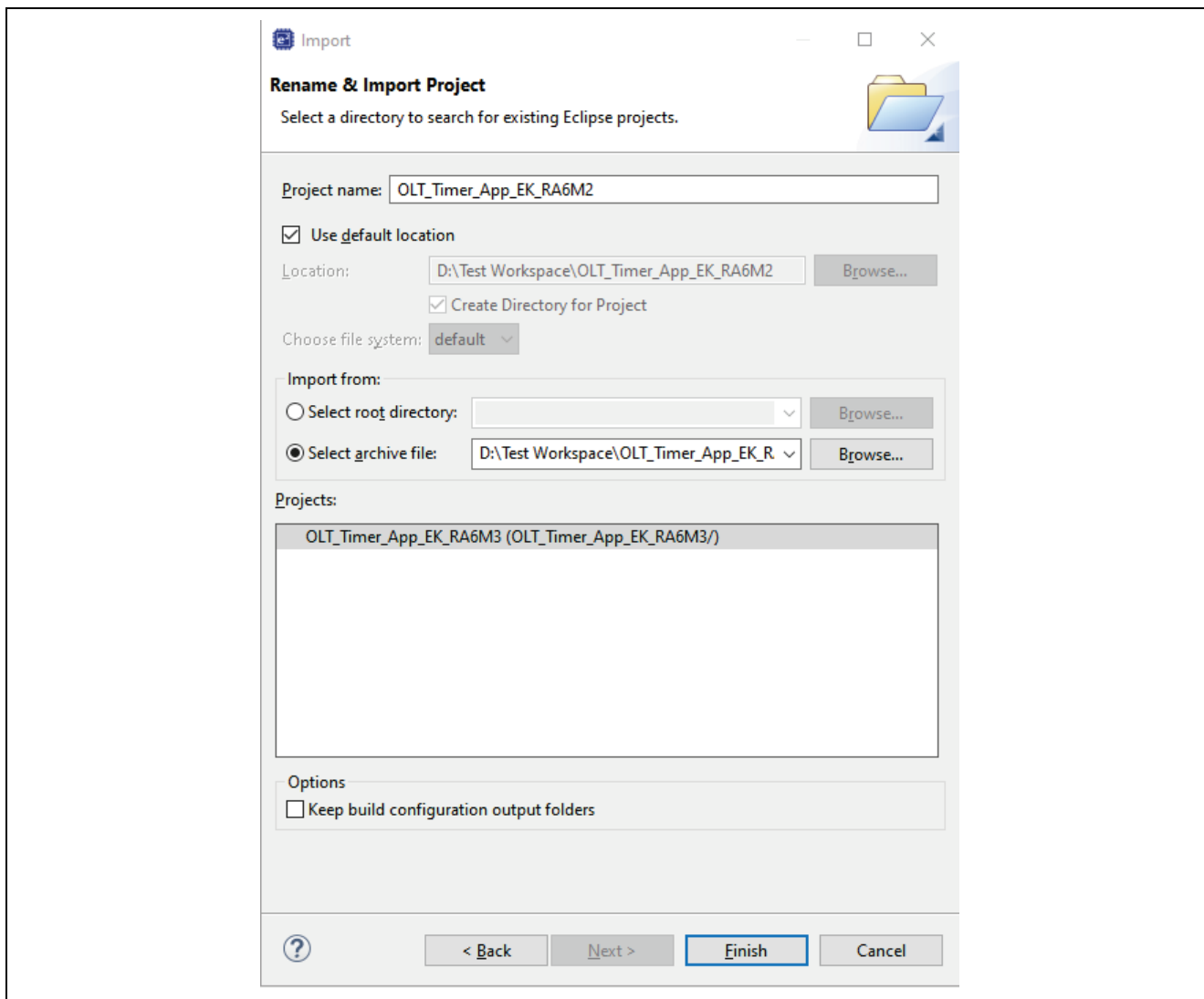
Figure 33. Rename and Import Project into e 2 studio
