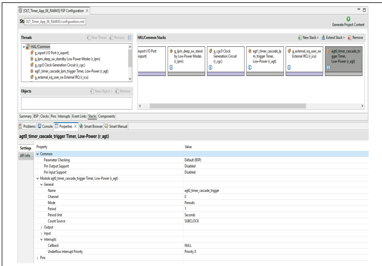
Figure 14. AGT0 Properties Configuration using the Properties Tab
