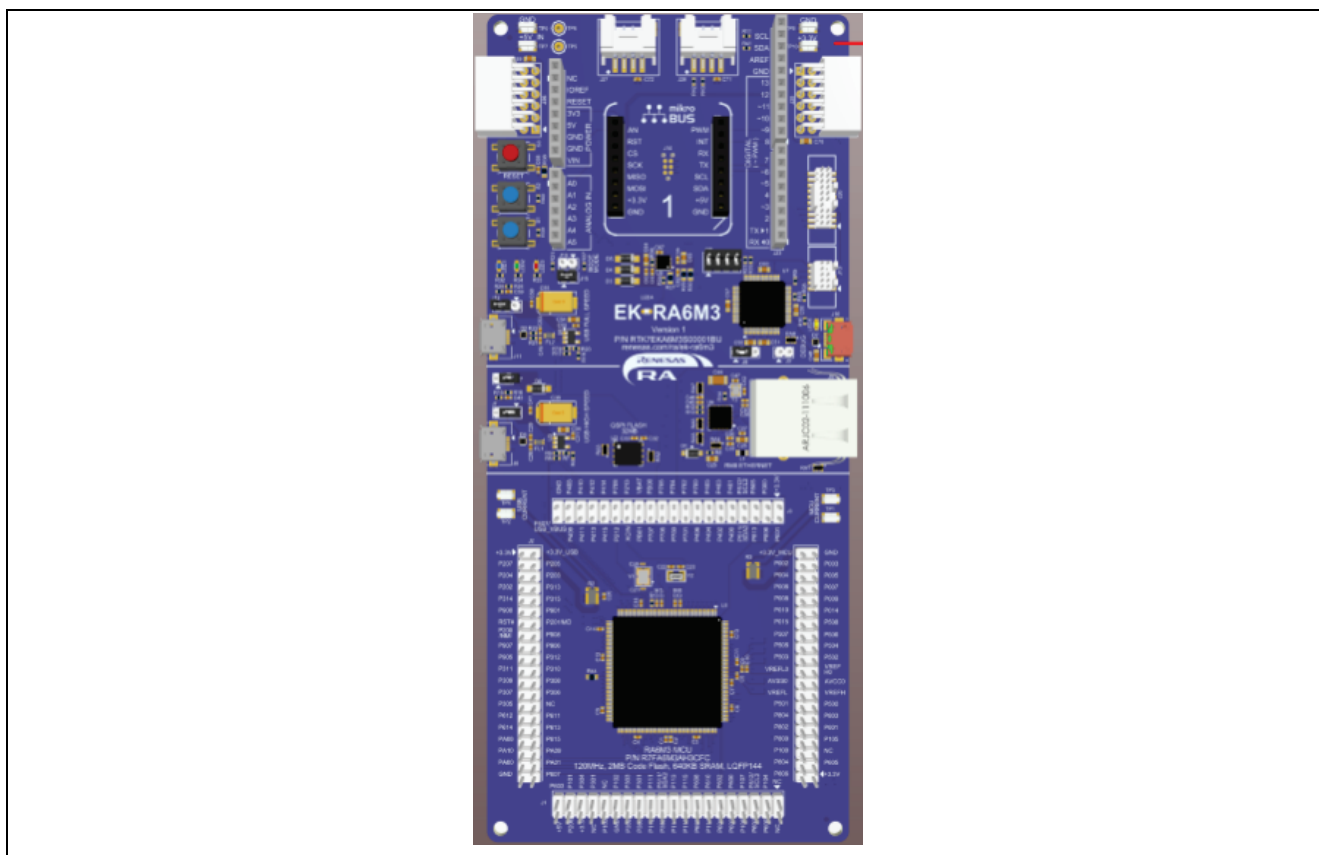
Figure 29. EK-RA6M3 Kit
