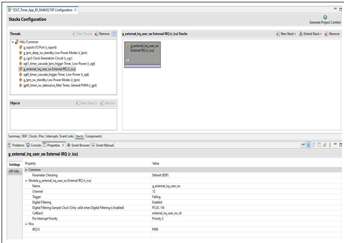
Figure 40. Change Peripheral Configuration
