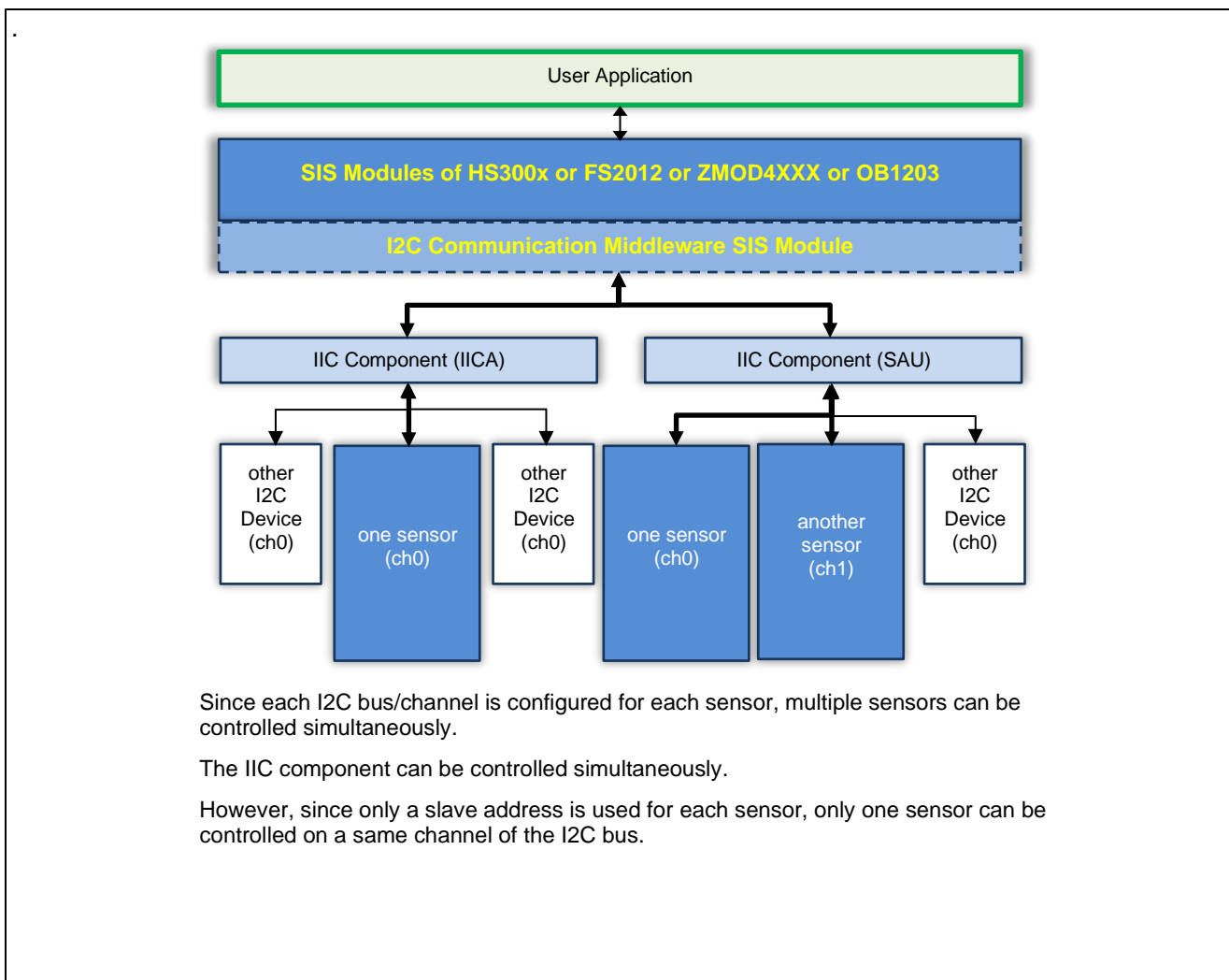
Figure 1-2 Example of Combination of Sensor (HS300x or FS2012 or ZMOD4410 or ZMOD4450 or ZMOD4510 or OB1203) SIS Modules and IIC Components
