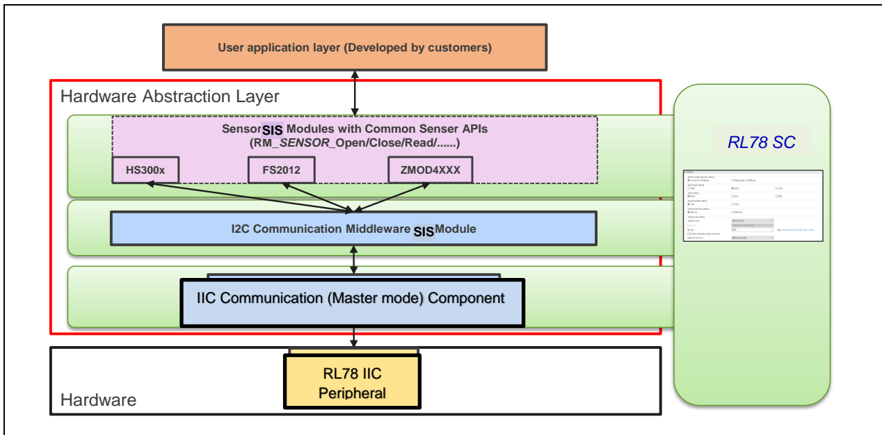
Figure 1-1 Renesas sensor software architecture
