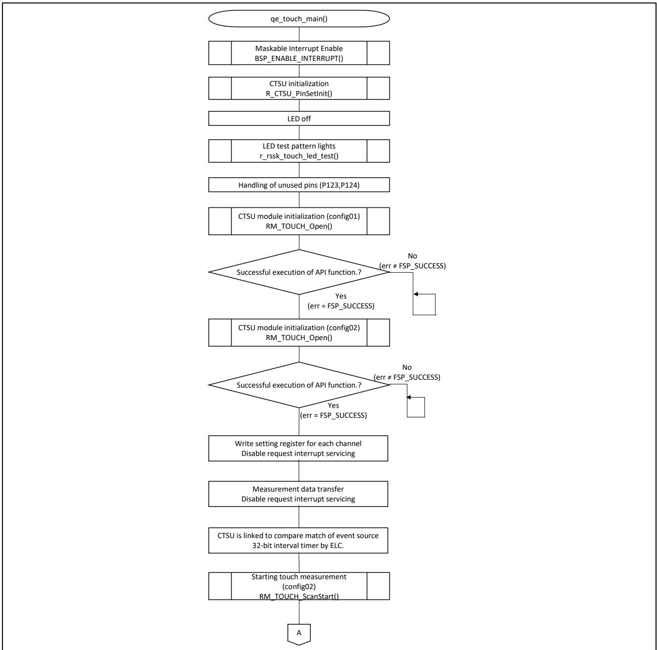
Figure 7-2 Touch measurement initial processing (1/3)
