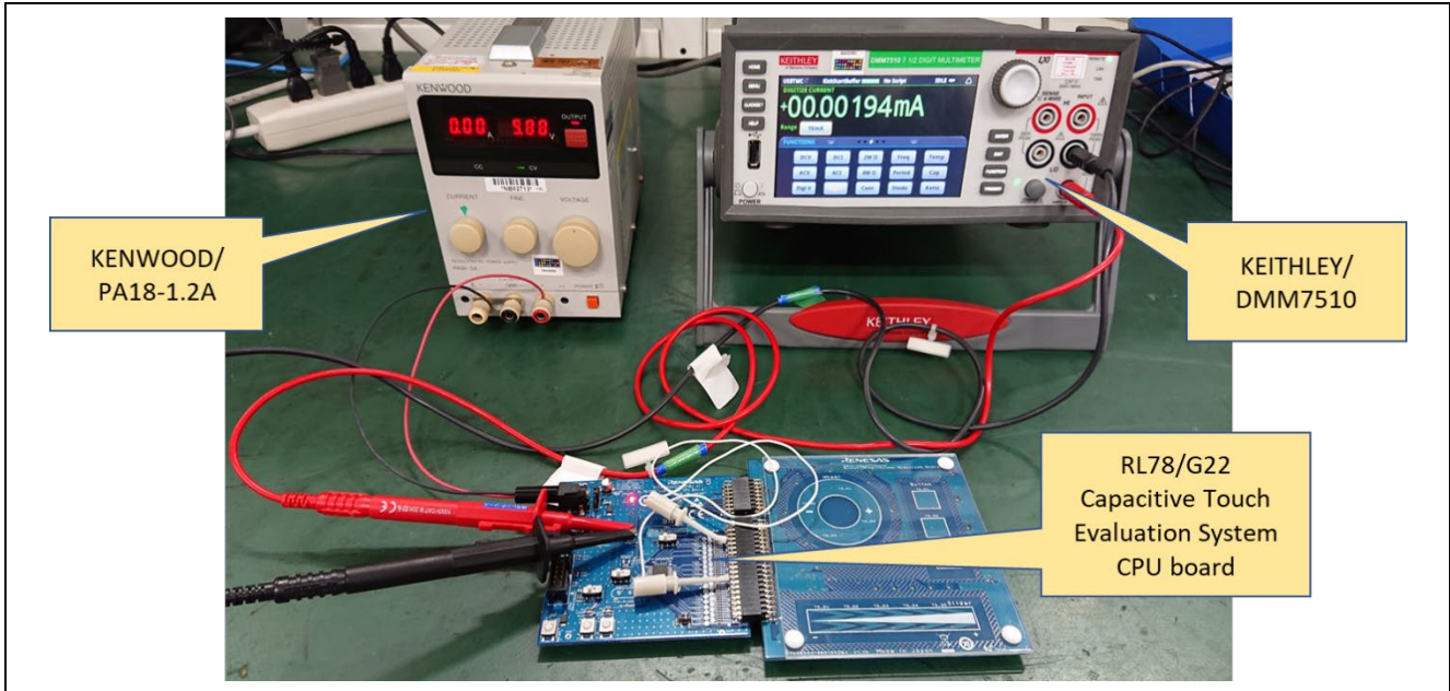
Figure 8-1 Environment to measure current consumption
