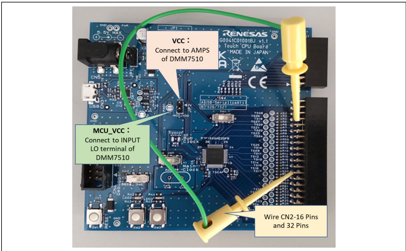
Figure 8-4 Pins of CPU board connected to the digital multimeter
