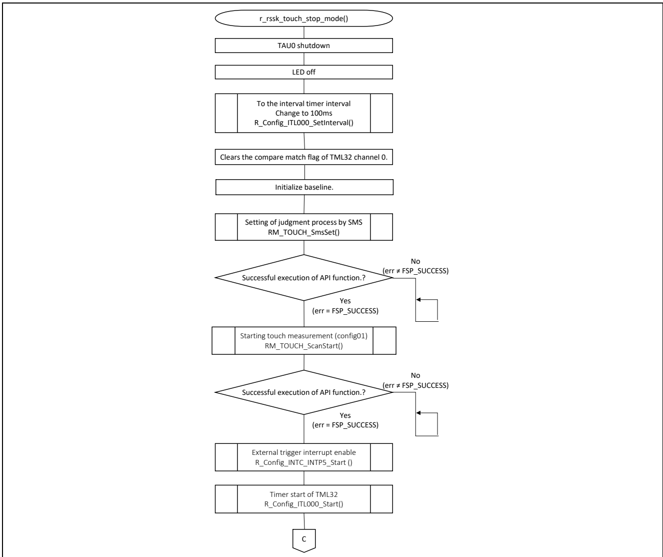
Figure 7-5 Touch Measurement Control Processing in Low Power Consumption Mode (1/2)
