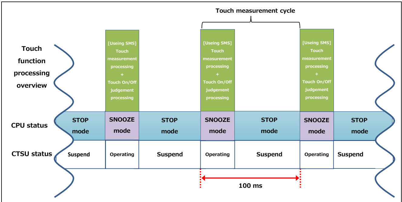
Figure 6-1 Operation image when measuring touch using SMS (When determining touch-off)
