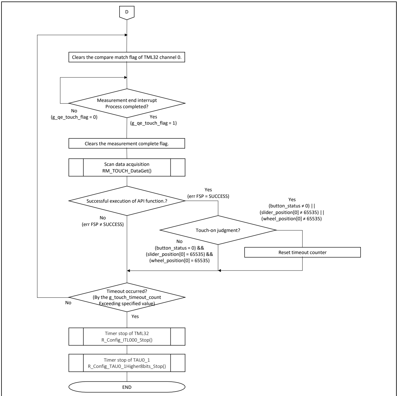
Figure 7-8 Touch Measurement Control Processing in Normal Mode (2/2)
