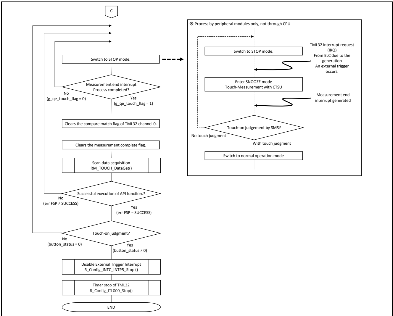
Figure 7-6 Touch Measurement Control Processing in Low Consumption Mode (2/2)
