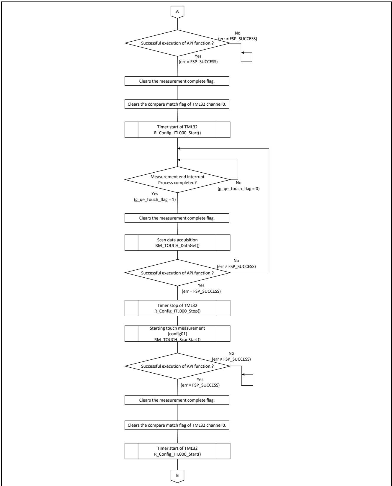
Figure 7-3 Touch measurement initial processing (2/3)
