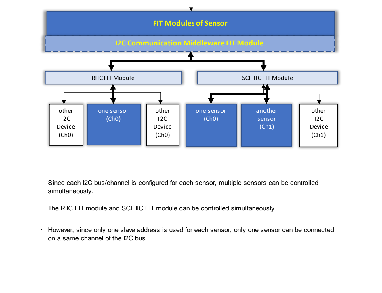
Figure 1-2 Example of Combination of Sensor FIT Modules and IIC FIT Modules
