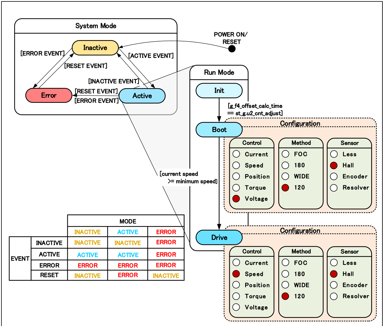
Figure 3-5 State Transition Diagram of 120-degree Conducting Control using hall sensors Software
