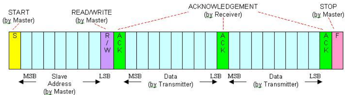
Figure 4: I2C Communication
