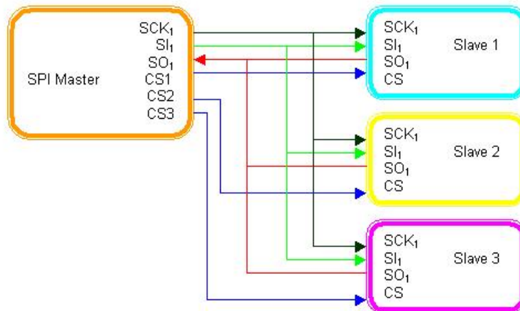
Figure 2: Single master, multiple slave SPI implementation
