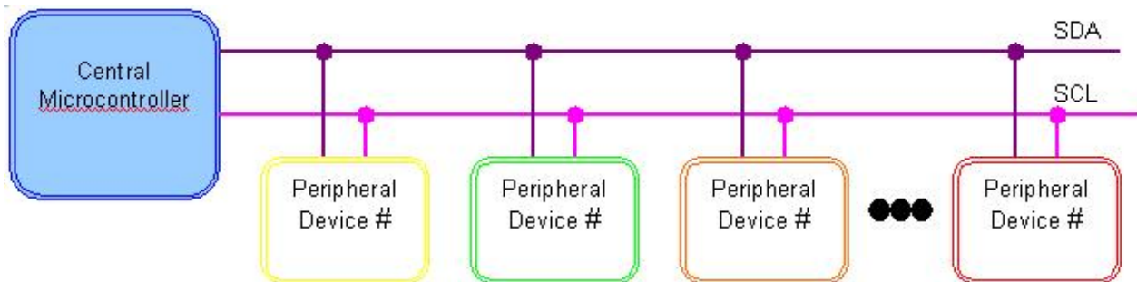
Figure 3: I 2 C has two lines in total
