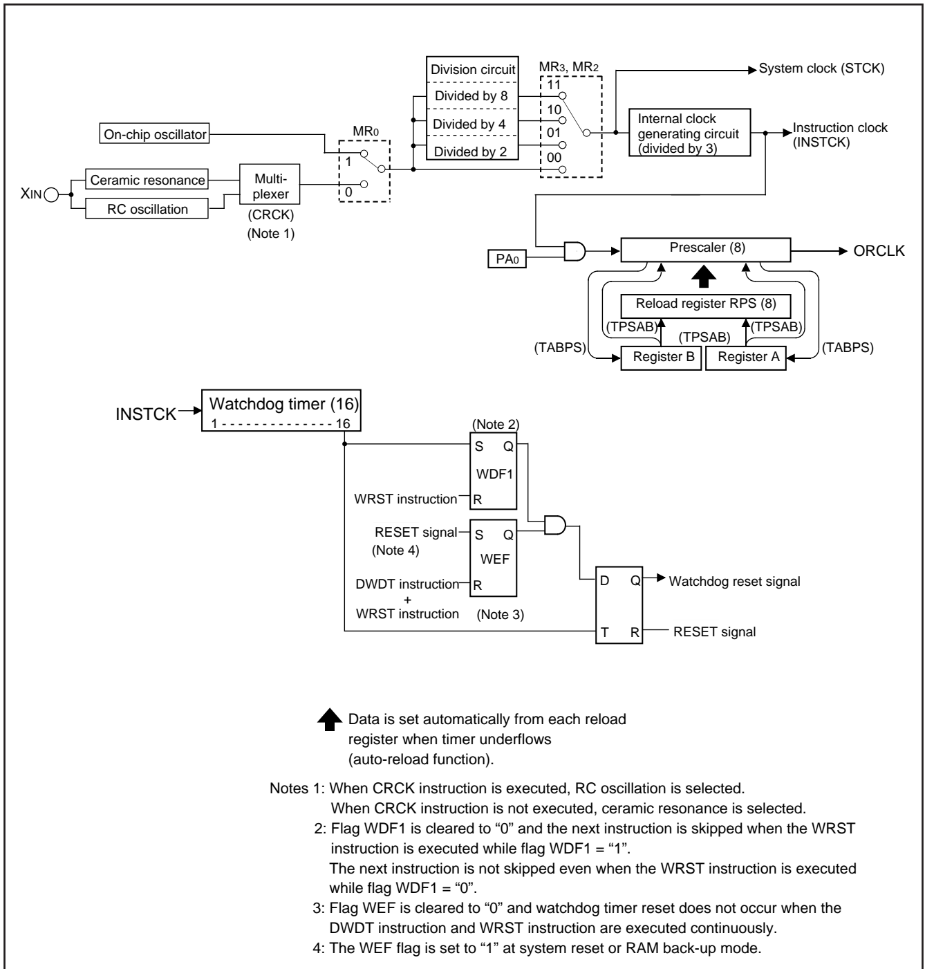
Fig. 22 Timers structure (1)
