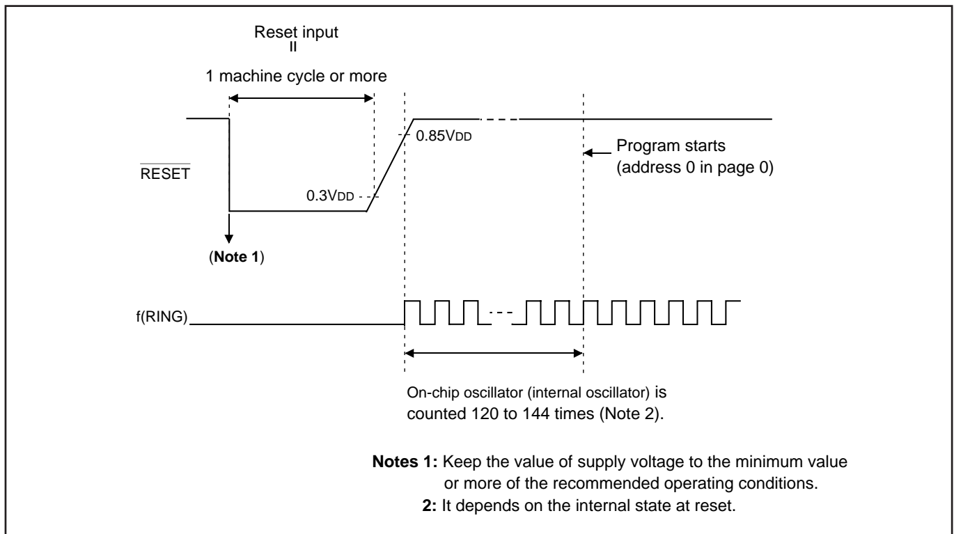
Fig. 41 \overline{\text{RESET}} pin input waveform and reset release timing
