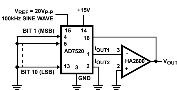
FIGURE 6. FEEDTHROUGH ERROR
