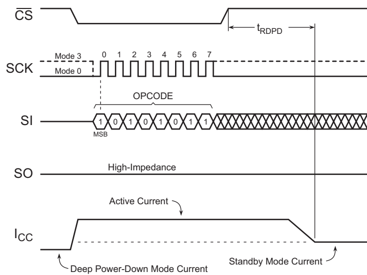
Figure 37. Resume from Deep Power-Down
