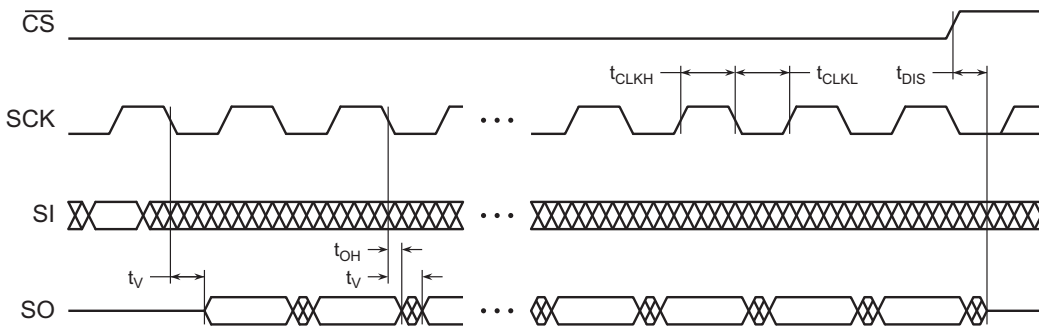
Figure 41. Serial Output Timing
