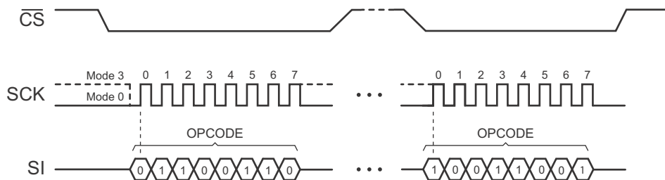
Figure 23. Enable Reset (66h) and Reset Device (99h) Command Timing (SPI Mode)
