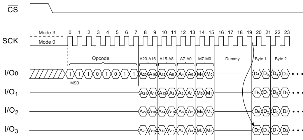
Figure 12. Quad-I/O Read Array (Initial command or previous M5, M4 ≠ 1,0)
