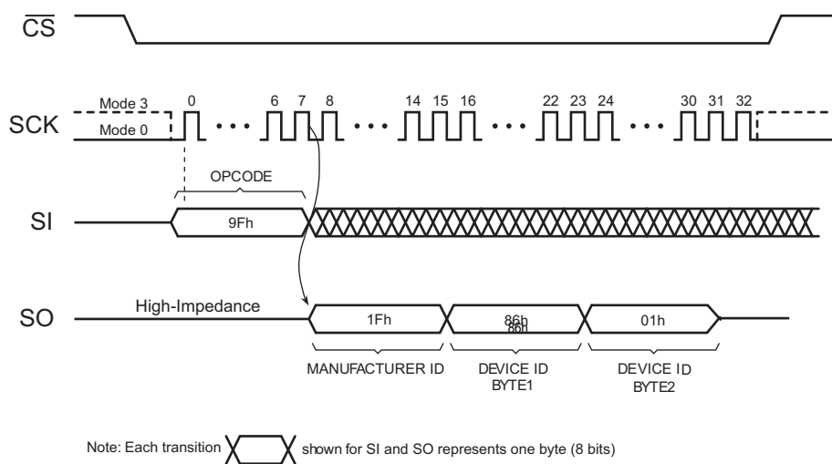
Figure 32. Read Manufacturer and Device ID
