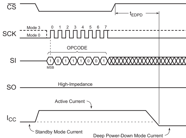
Figure 36. Deep Power-Down
