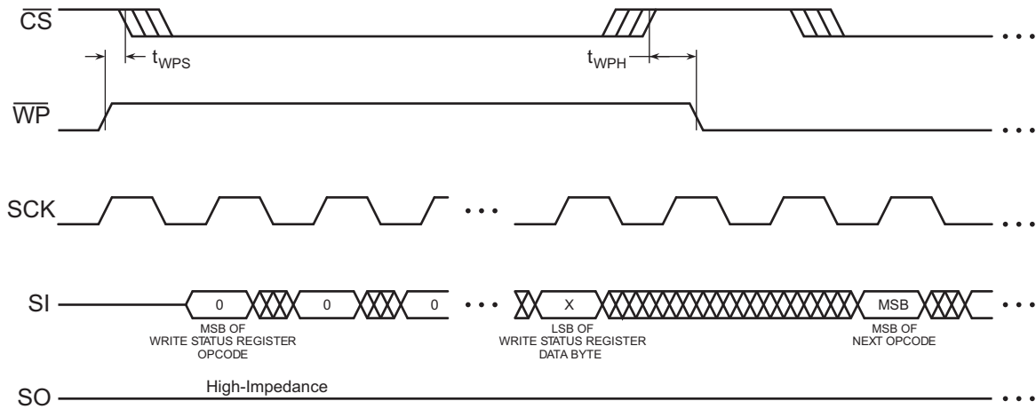
Figure 42. \overline{WP} Timing for Write Status Register Command When BPL = 1
