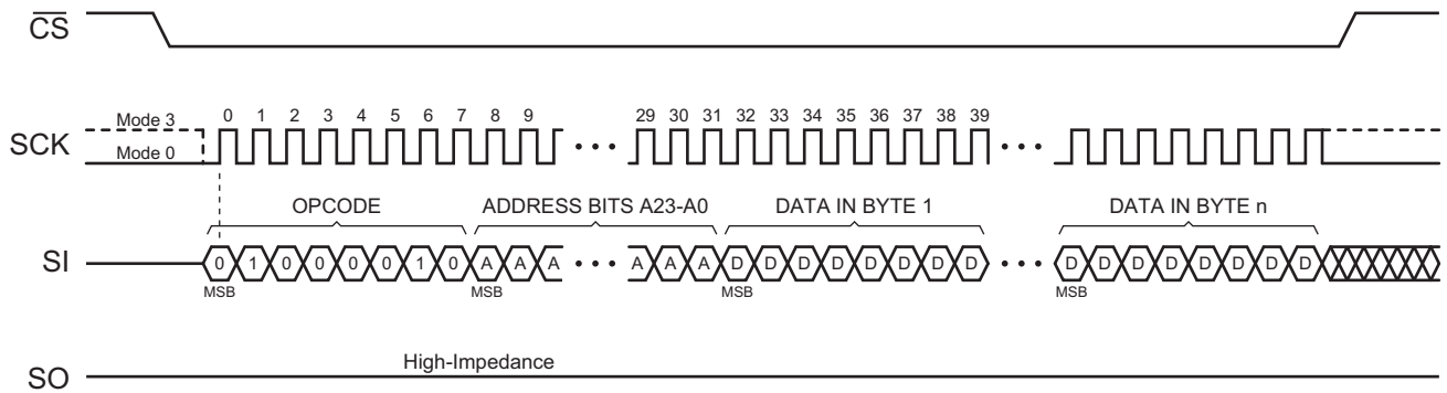
Figure 26. Program Security Registers
