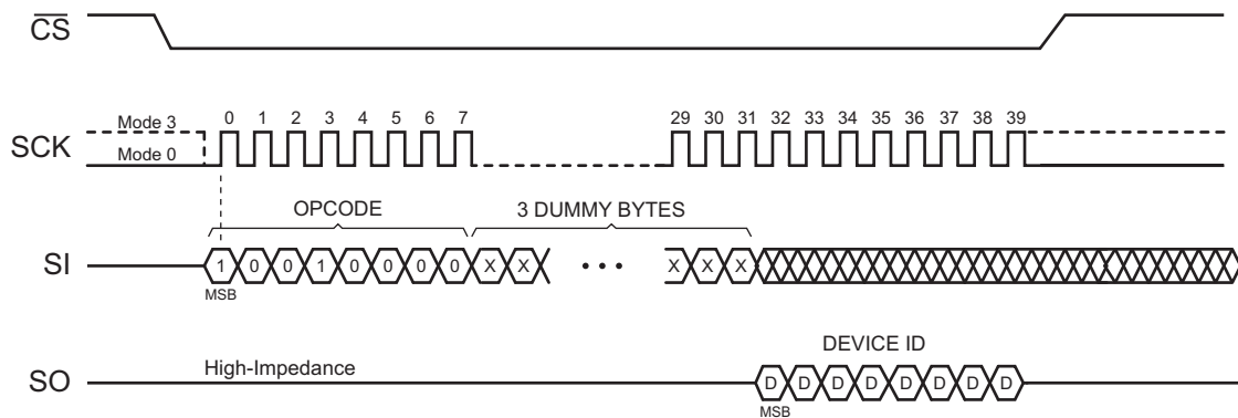
Figure 33. Read ID (Legacy Command)
