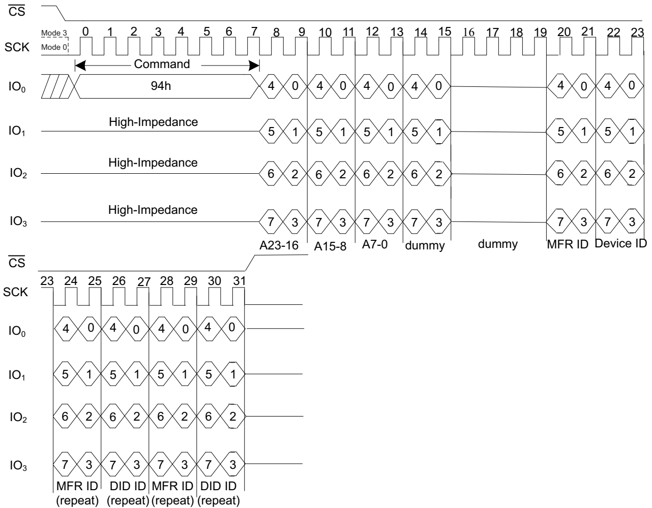
Figure 35. Quad I/O Read Manufacturer ID / Device ID Timing
