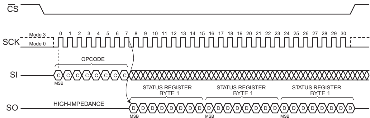
Figure 28. Read Status Register 1
