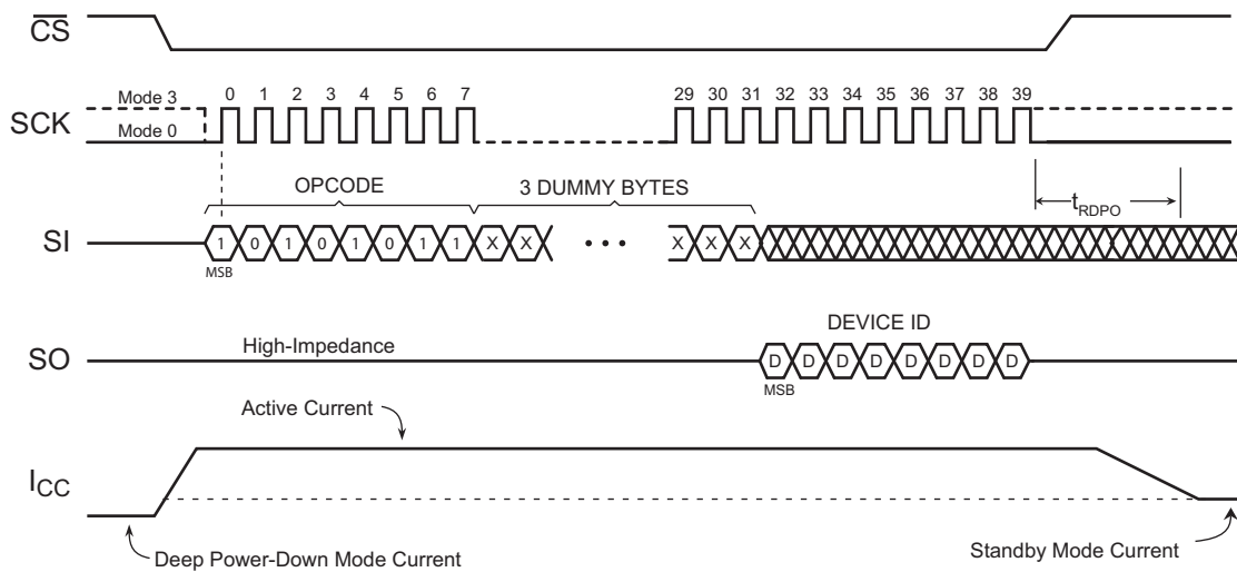
Figure 38. Resume from Deep Power-Down and Read Device ID Timing
