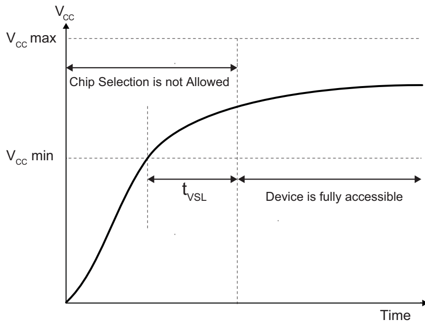
Figure 39. Power-Up Timing and Voltage
