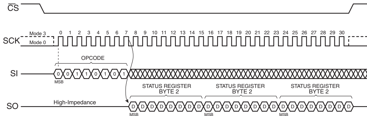
Figure 29. Read Status Register 2
