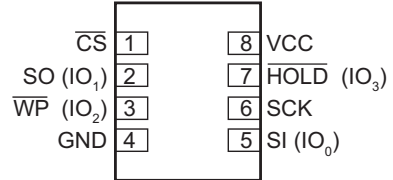
Figure 3. 8-DFN — Top View
