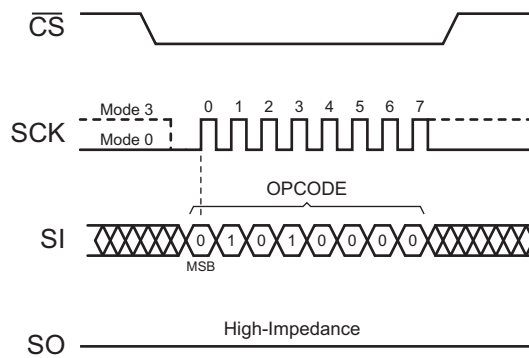
Figure 31. Write Enable for Volatile Status Register
