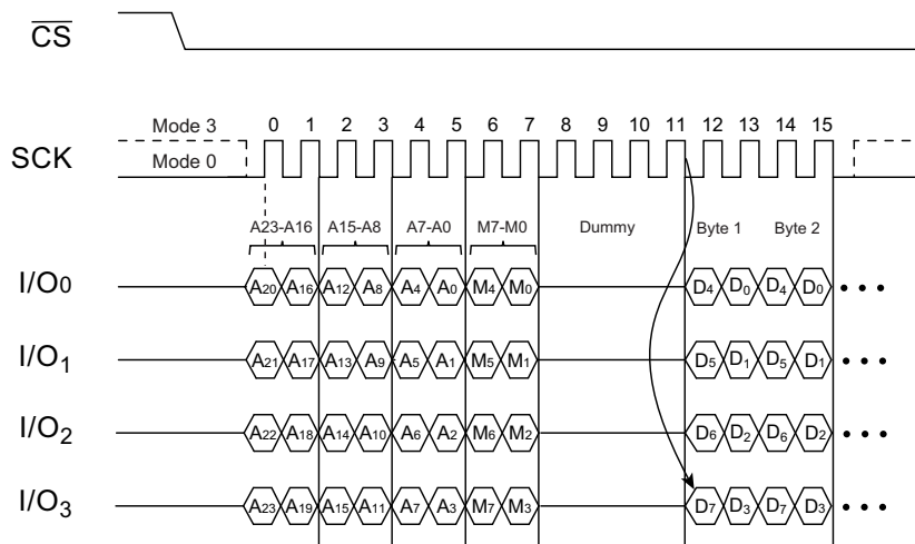
Figure 13. Quad I/O Read Array with Continuous Read Mode (Previous Command Set M5, M4 = 1,0)
