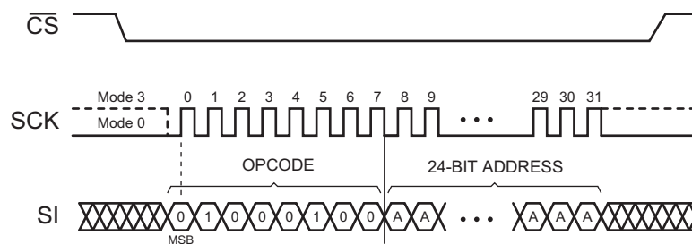
Figure 25. Erase Security Register Page
