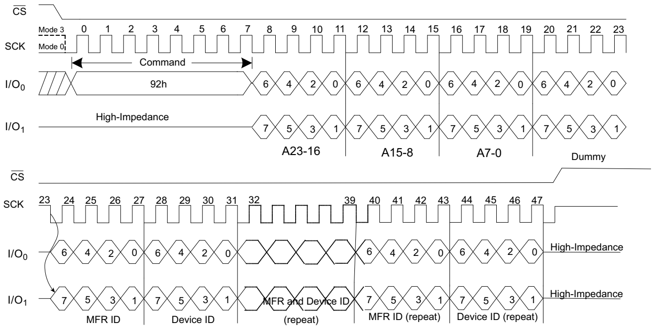
Figure 34. Dual I/O Read Manufacture ID/ Device ID Timing
