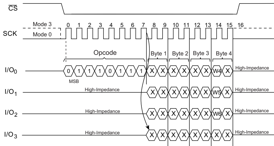
Figure 14. Set Burst with Wrap Timing (SPI Mode)
