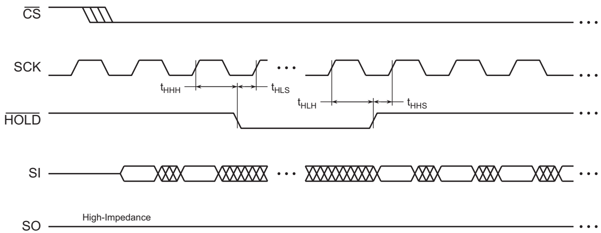
Figure 43. \overline{HOLD} Timing – Serial Input
