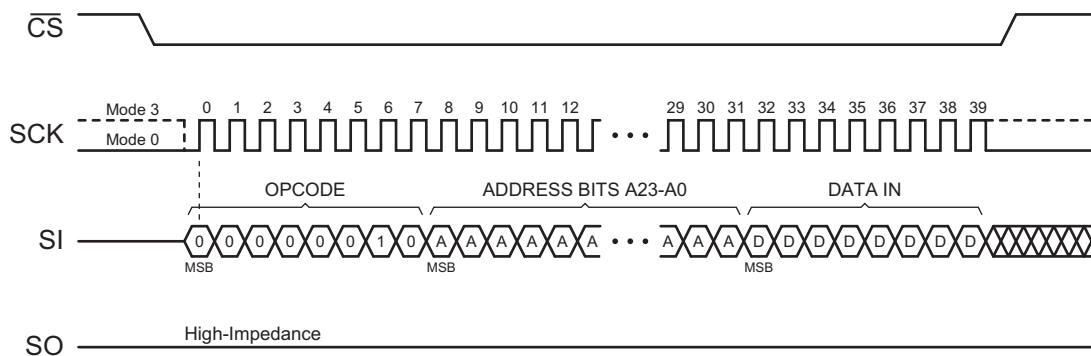
Figure 18. Byte Program
