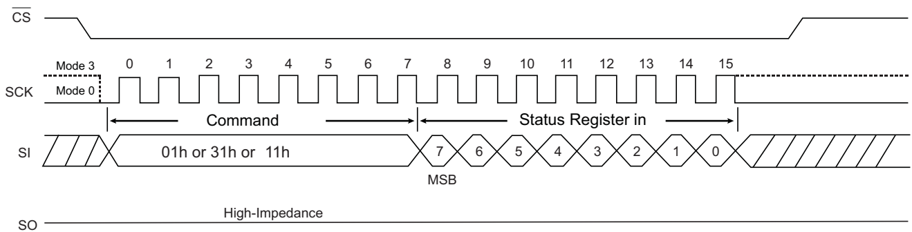
Figure 30. Write Status Register
