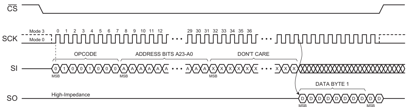
Figure 27. Read Security Registers
