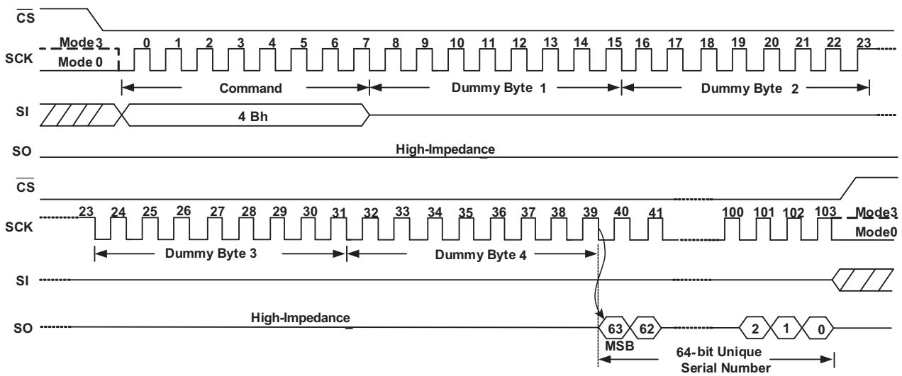
Figure 24. Read Unique ID Timing (SPI Mode)
