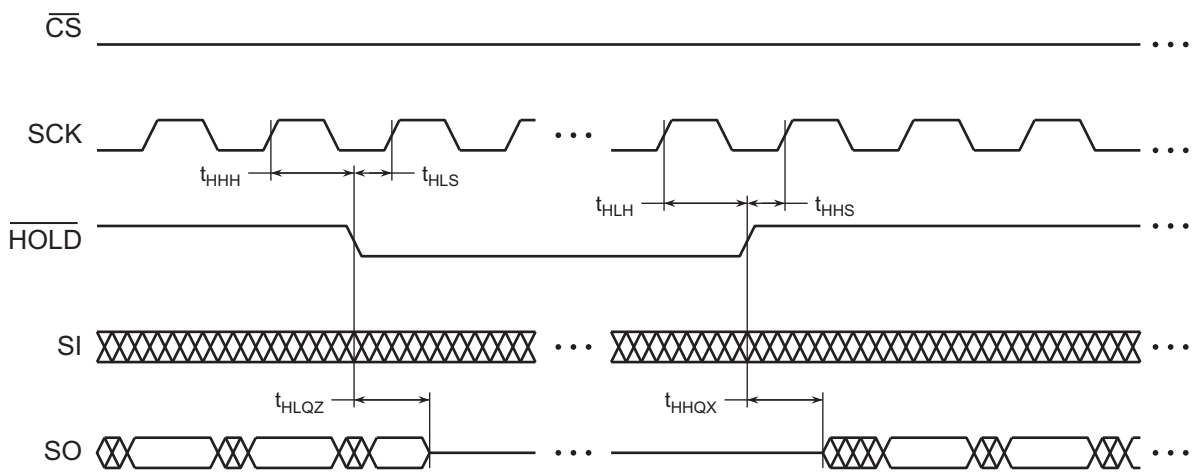
Figure 44. \overline{HOLD} Timing – Serial Output
